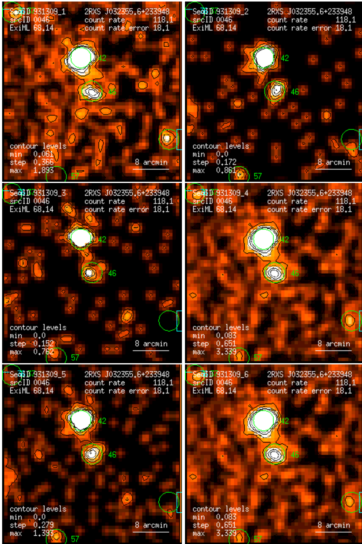
Figure 46: RASS 931309: detection 0046: band rate images, Gaussian filter: (1) PSPC channels 11 – 41, (2) 52 – 90, (3) 91 – 201, (4) 11 – 235, (5) 52 – 201, (6) 11 – 201. Broad band rates in counts/ks. Band rate contour levels in counts/ks/arcmin 2 .
