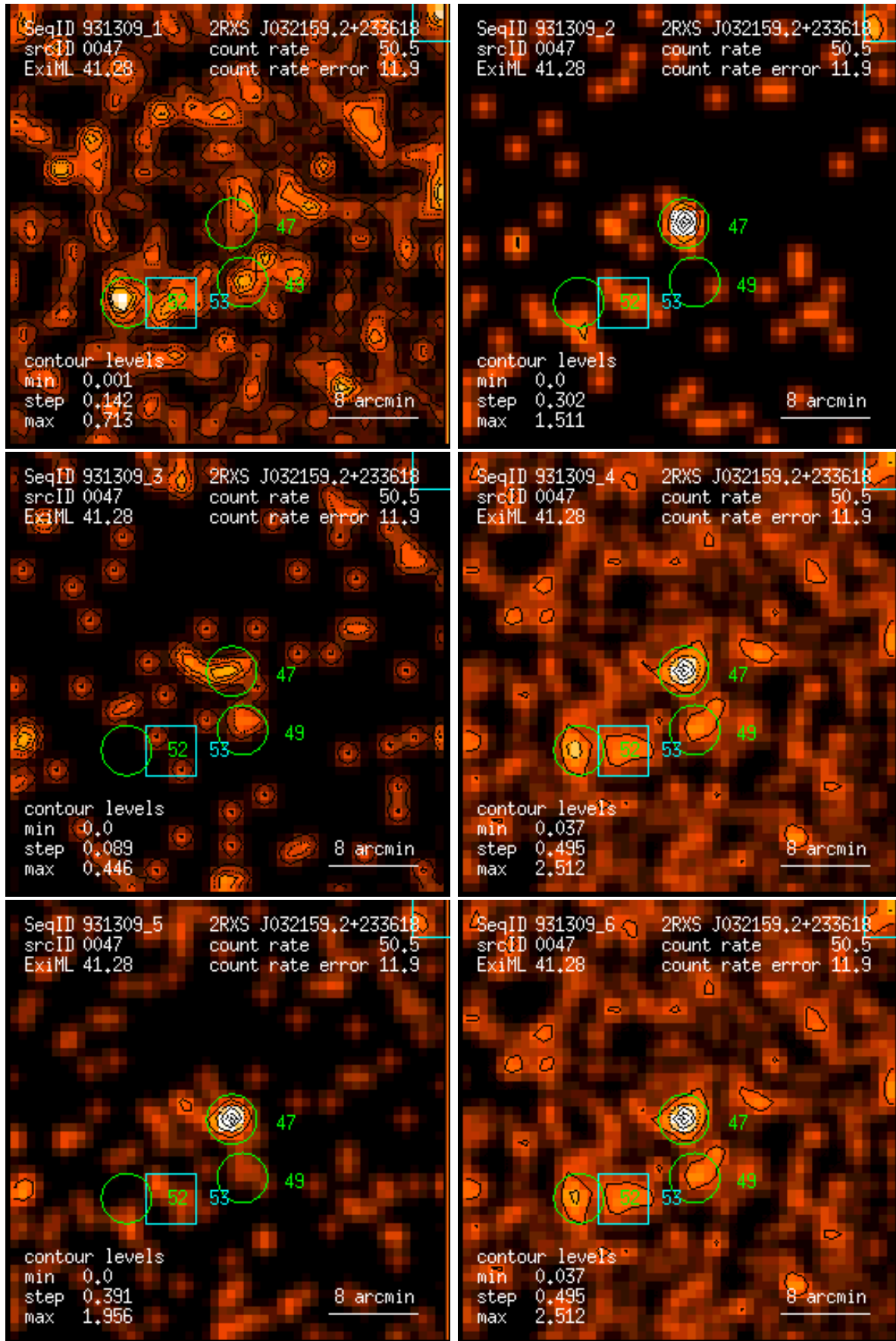
Figure 47: RASS 931309: detection 0047: band rate images, Gaussian filter: (1) PSPC channels 11 – 41, (2) 52 – 90, (3) 91 – 201, (4) 11 – 235, (5) 52 – 201, (6) 11 – 201. Broad band rates in counts/ks. Band rate contour levels in counts/ks/arcmin 2 .
