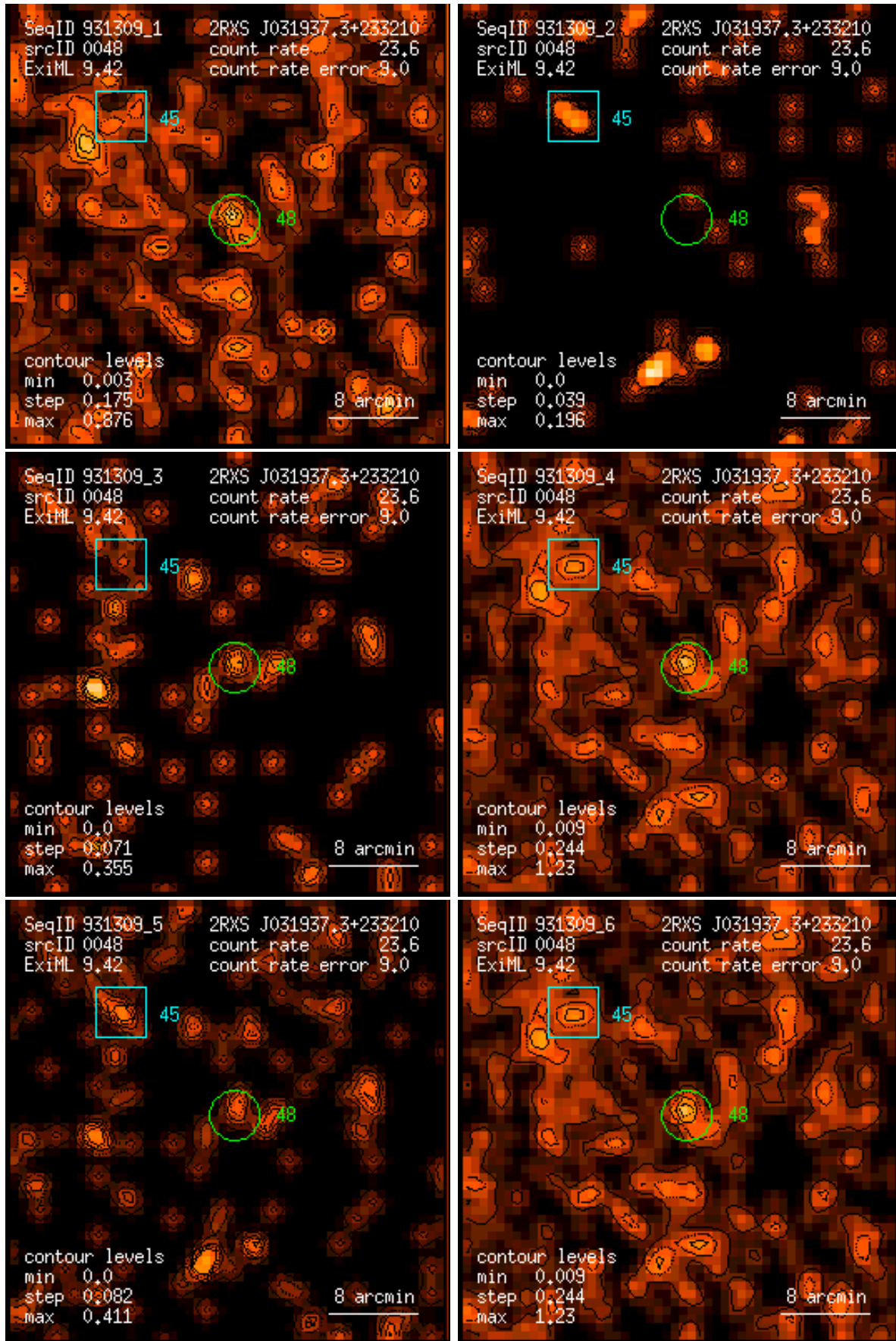
Figure 48: RASS 931309: detection 0048: band rate images, Gaussian filter: (1) PSPC channels 11 – 41, (2) 52 – 90, (3) 91 – 201, (4) 11 – 235, (5) 52 – 201, (6) 11 – 201. Broad band rates in counts/ks. Band rate contour levels in counts/ks/arcmin 2 .
