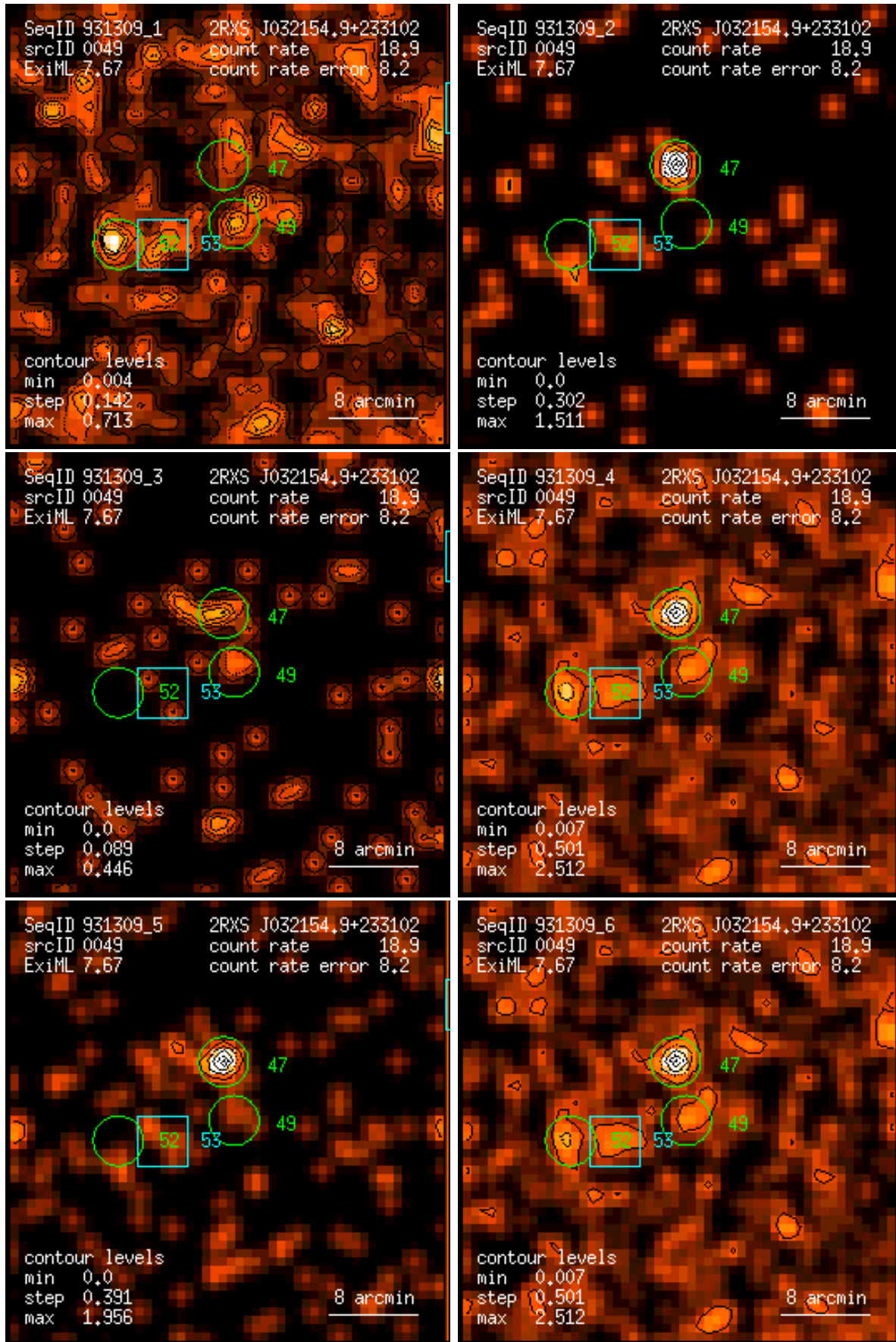
Figure 49: RASS 931309: detection 0049: band rate images, Gaussian filter: (1) PSPC channels 11 – 41, (2) 52 – 90, (3) 91 – 201, (4) 11 – 235, (5) 52 – 201, (6) 11 – 201. Broad band rates in counts/ks. Band rate contour levels in counts/ks/arcmin 2 .
