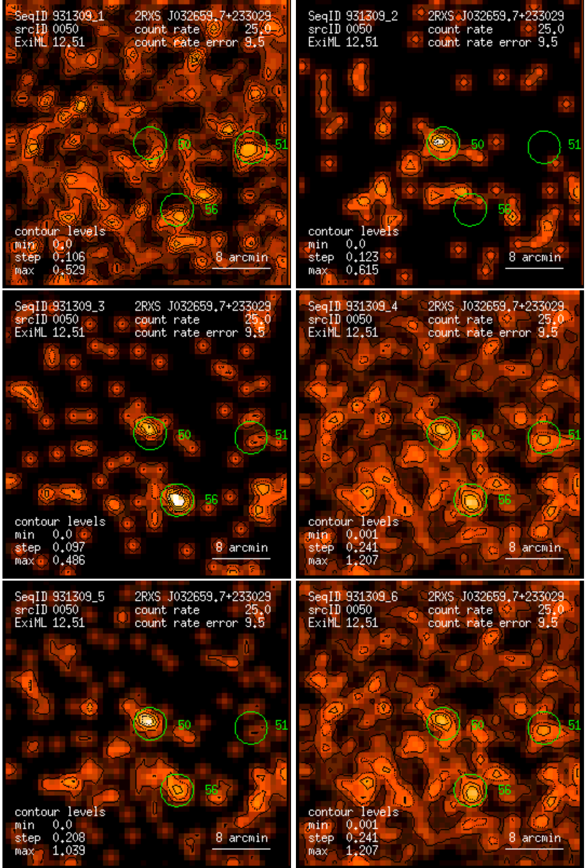
Figure 50: RASS 931309: detection 0050: band rate images, Gaussian filter: (1) PSPC channels 11 – 41, (2) 52 – 90, (3) 91 – 201, (4) 11 – 235, (5) 52 – 201, (6) 11 – 201. Broad band rates in counts/ks. Band rate contour levels in counts/ks/arcmin 2 .
