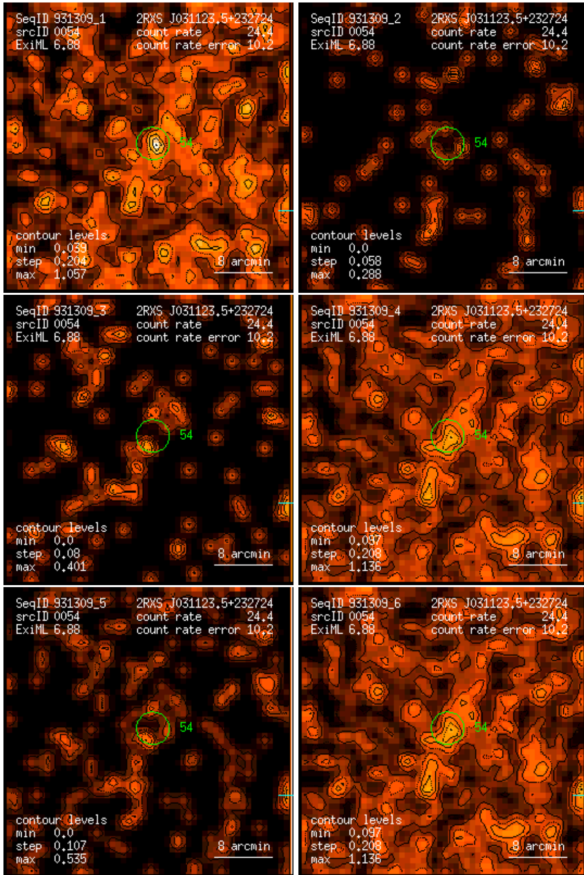
Figure 54: RASS 931309: detection 0054: band rate images, Gaussian filter: (1) PSPC channels 11 – 41, (2) 52 – 90, (3) 91 – 201, (4) 11 – 235, (5) 52 – 201, (6) 11 – 201. Broad band rates in counts/ks. Band rate contour levels in counts/ks/arcmin 2 .
