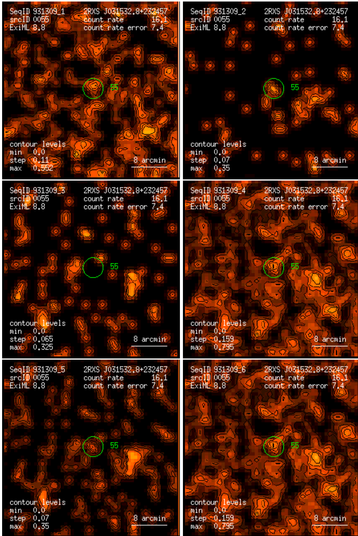
Figure 55: RASS 931309: detection 0055: band rate images, Gaussian filter: (1) PSPC channels 11 – 41, (2) 52 – 90, (3) 91 – 201, (4) 11 – 235, (5) 52 – 201, (6) 11 – 201. Broad band rates in counts/ks. Band rate contour levels in counts/ks/arcmin 2 .
