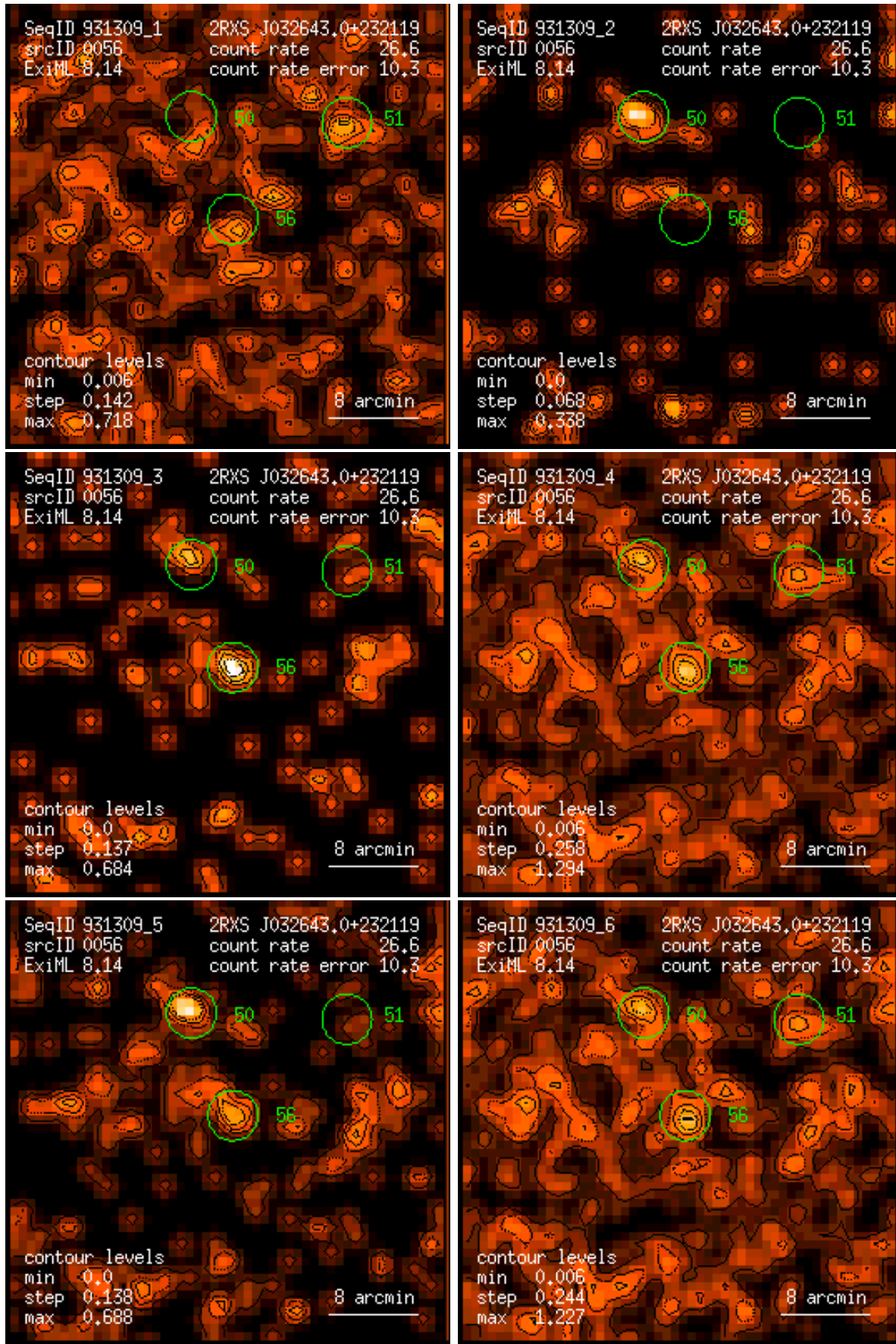
Figure 56: RASS 931309: detection 0056: band rate images, Gaussian filter: (1) PSPC channels 11 – 41, (2) 52 – 90, (3) 91 – 201, (4) 11 – 235, (5) 52 – 201, (6) 11 – 201. Broad band rates in counts/ks. Band rate contour levels in counts/ks/arcmin 2 .
