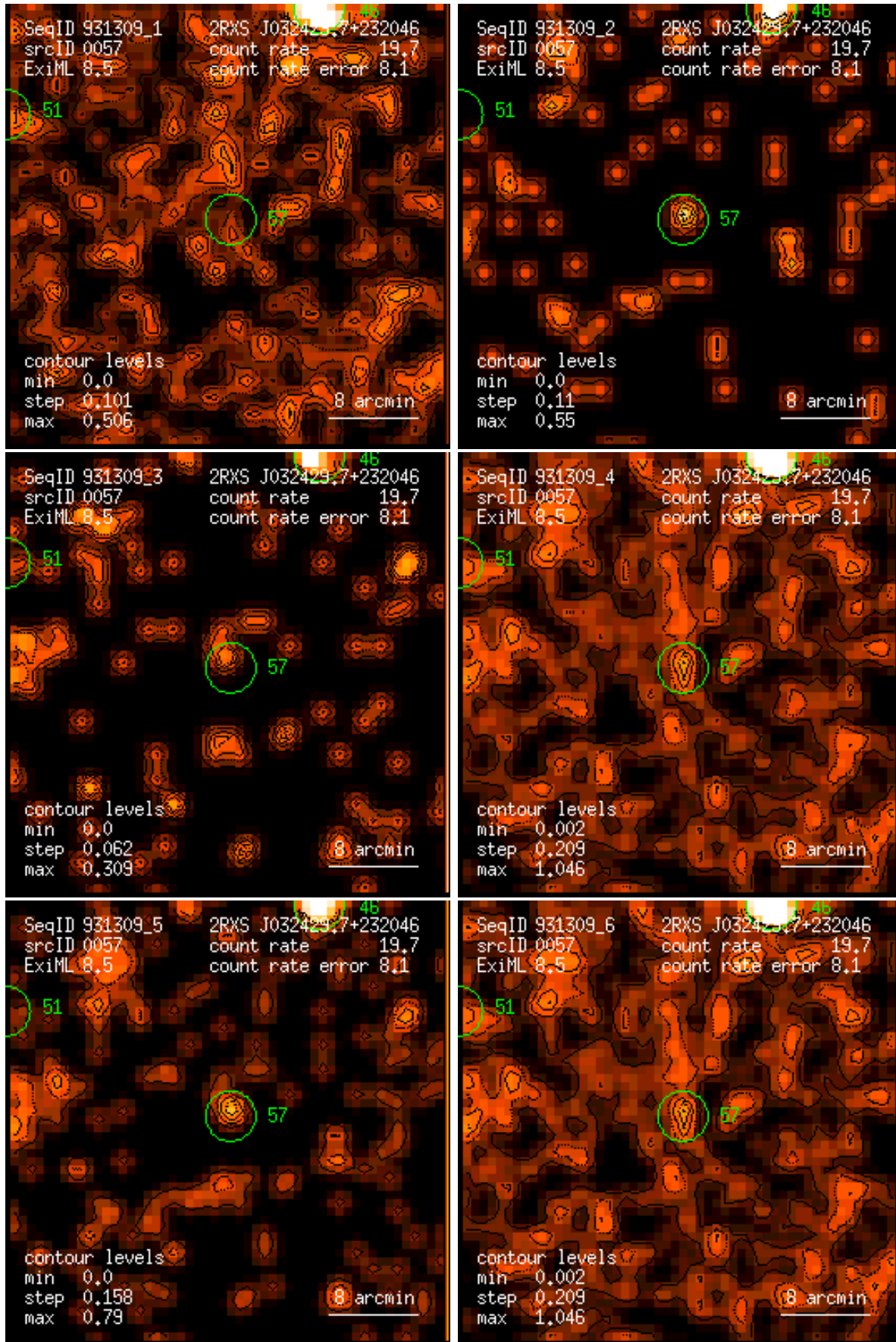
Figure 57: RASS 931309: detection 0057: band rate images, Gaussian filter: (1) PSPC channels 11 – 41, (2) 52 – 90, (3) 91 – 201, (4) 11 – 235, (5) 52 – 201, (6) 11 – 201. Broad band rates in counts/ks. Band rate contour levels in counts/ks/arcmin 2 .
