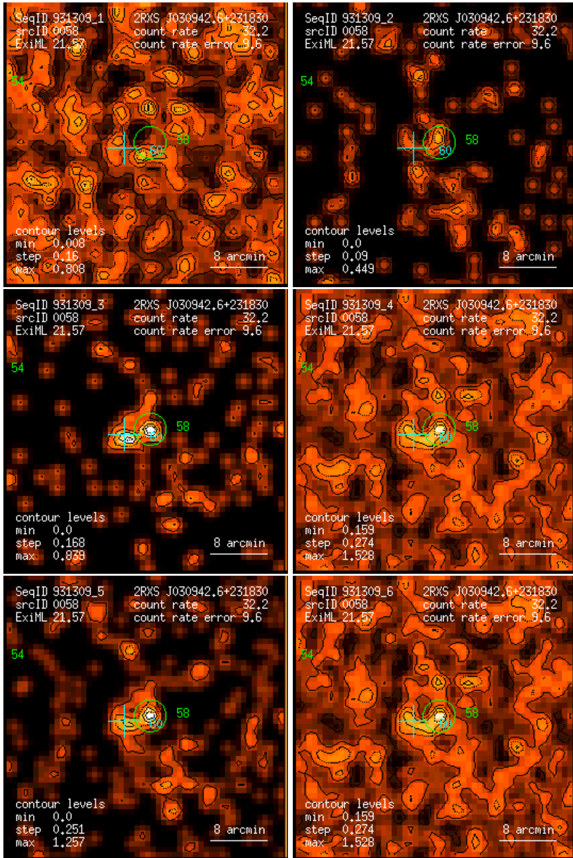
Figure 58: RASS 931309: detection 0058: band rate images, Gaussian filter: (1) PSPC channels 11 – 41, (2) 52 – 90, (3) 91 – 201, (4) 11 – 235, (5) 52 – 201, (6) 11 – 201. Broad band rates in counts/ks. Band rate contour levels in counts/ks/arcmin 2 .
