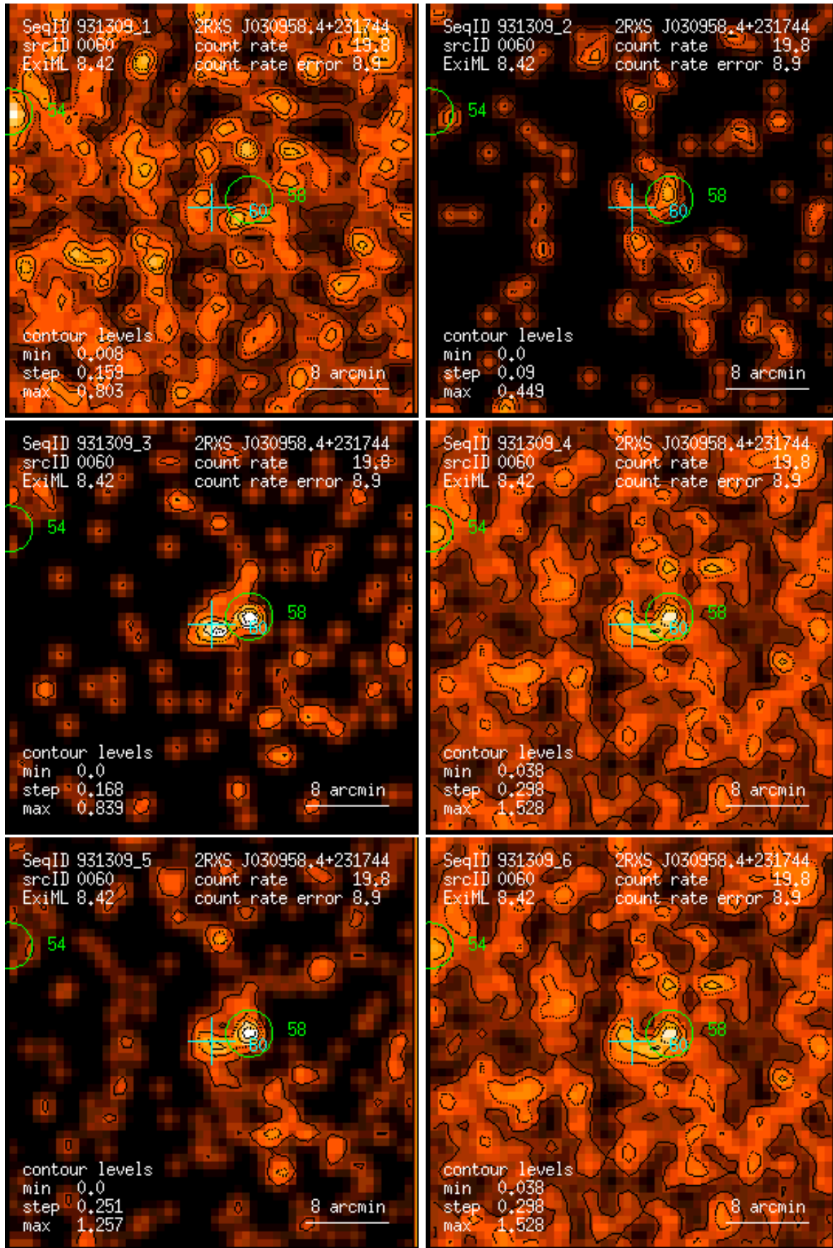
Figure 60: RASS 931309: detection 0060: band rate images, Gaussian filter: (1) PSPC channels 11 – 41, (2) 52 – 90, (3) 91 – 201, (4) 11 – 235, (5) 52 – 201, (6) 11 – 201. Broad band rates in counts/ks. Band rate contour levels in counts/ks/arcmin 2 .
