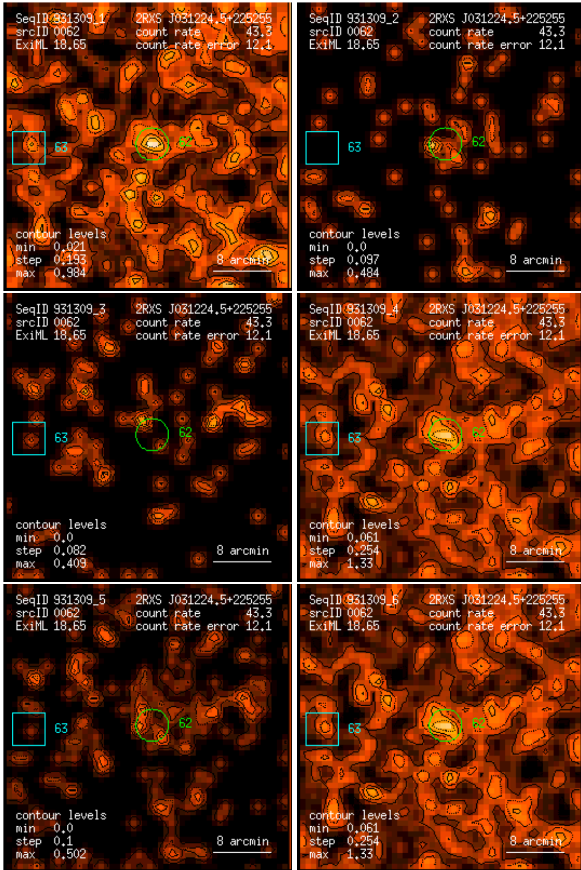
Figure 62: RASS 931309: detection 0062: band rate images, Gaussian filter: (1) PSPC channels 11 – 41, (2) 52 – 90, (3) 91 – 201, (4) 11 – 235, (5) 52 – 201, (6) 11 – 201. Broad band rates in counts/ks. Band rate contour levels in counts/ks/arcmin 2 .
