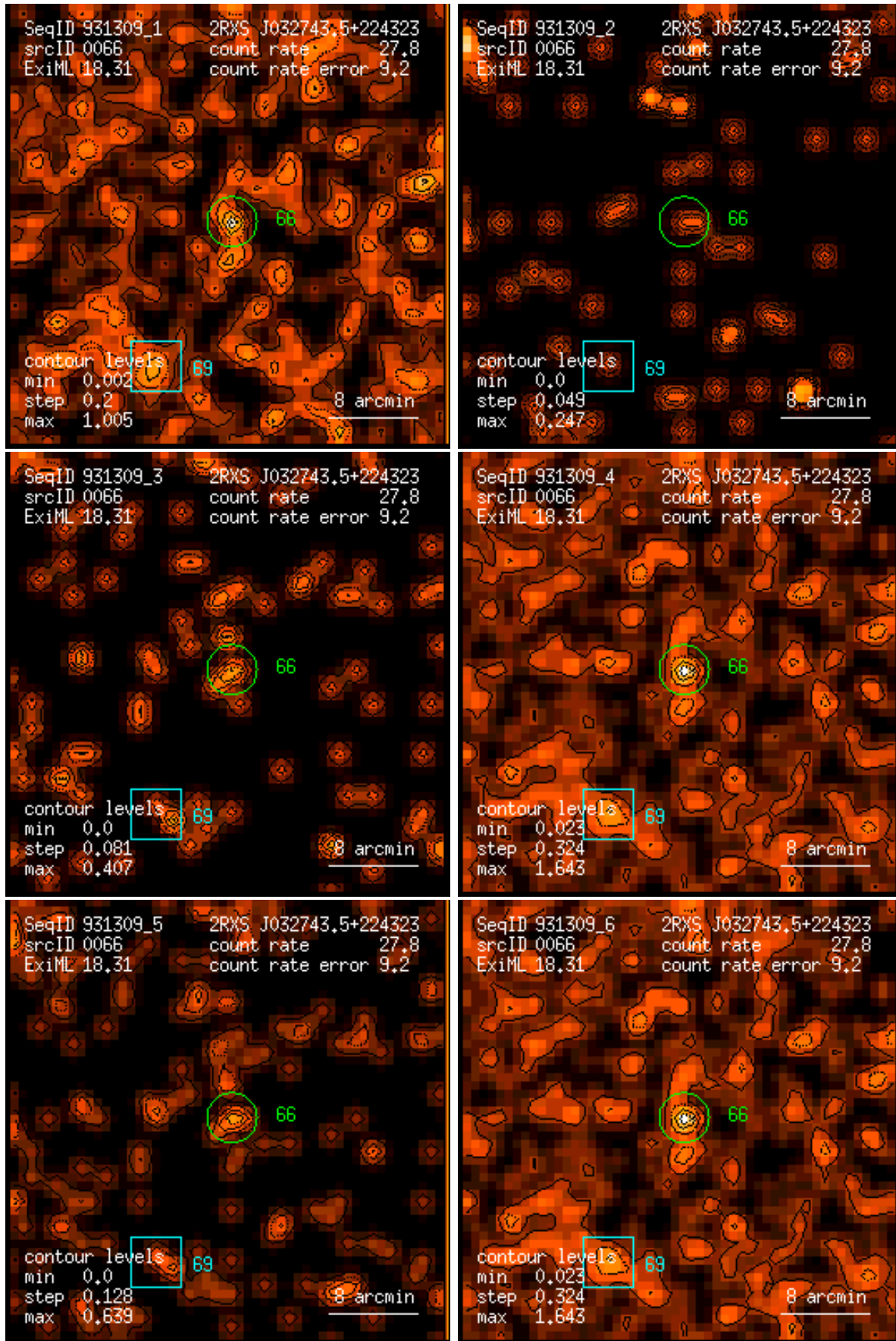
Figure 66: RASS 931309: detection 0066: band rate images, Gaussian filter: (1) PSPC channels 11 – 41, (2) 52 – 90, (3) 91 – 201, (4) 11 – 235, (5) 52 – 201, (6) 11 – 201. Broad band rates in counts/ks. Band rate contour levels in counts/ks/arcmin 2 .
