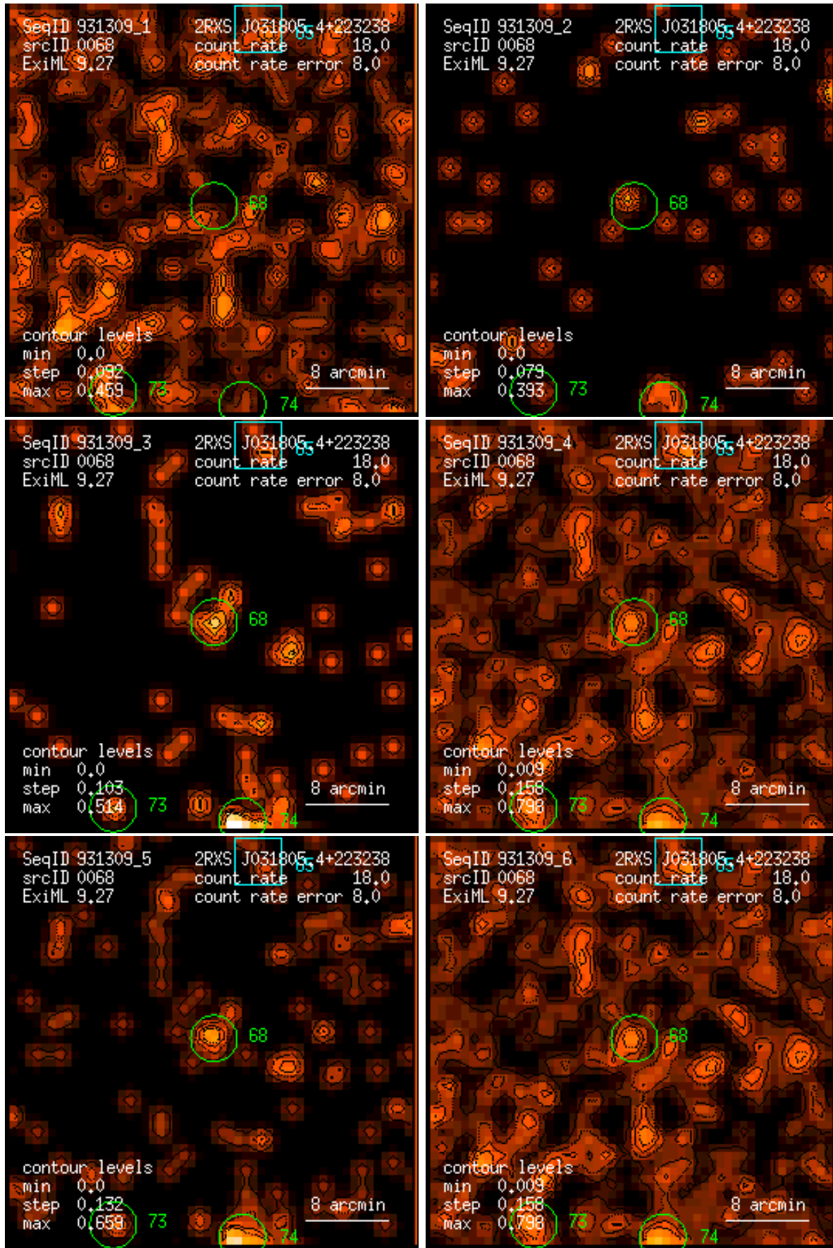
Figure 68: RASS 931309: detection 0068: band rate images, Gaussian filter: (1) PSPC channels 11 – 41, (2) 52 – 90, (3) 91 – 201, (4) 11 – 235, (5) 52 – 201, (6) 11 – 201. Broad band rates in counts/ks. Band rate contour levels in counts/ks/arcmin 2 .
