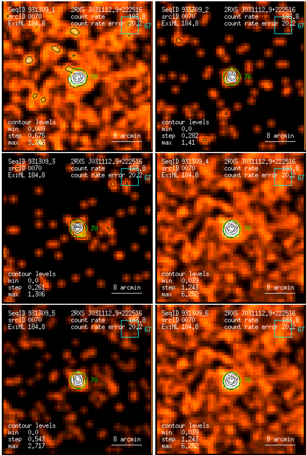
Figure 70: RASS 931309: detection 0070: band rate images, Gaussian filter: (1) PSPC channels 11 – 41, (2) 52 – 90, (3) 91 – 201, (4) 11 – 235, (5) 52 – 201, (6) 11 – 201. Broad band rates in counts/ks. Band rate contour levels in counts/ks/arcmin 2 .
