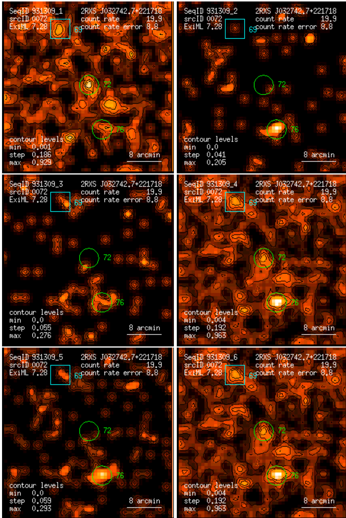
Figure 72: RASS 931309: detection 0072: band rate images, Gaussian filter: (1) PSPC channels 11 – 41, (2) 52 – 90, (3) 91 – 201, (4) 11 – 235, (5) 52 – 201, (6) 11 – 201. Broad band rates in counts/ks. Band rate contour levels in counts/ks/arcmin 2 .
