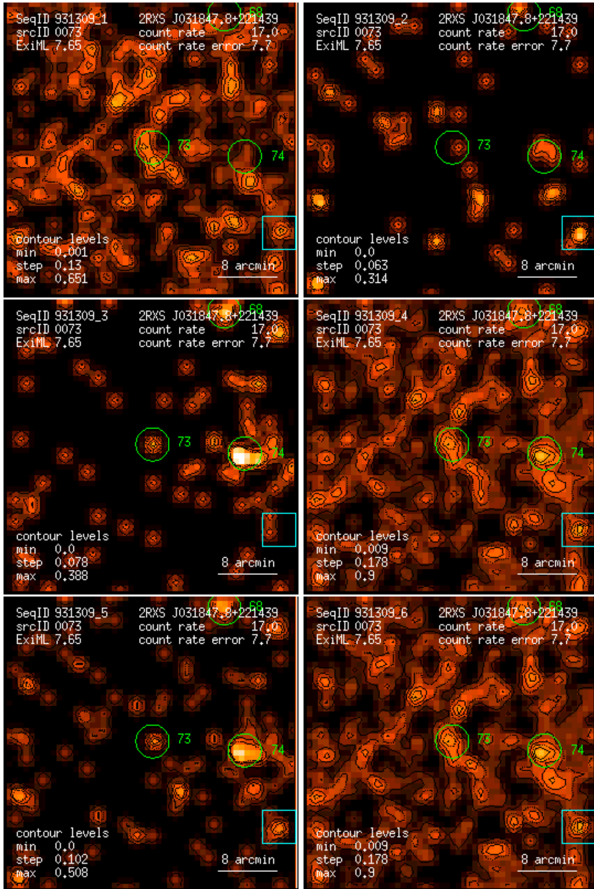
Figure 73: RASS 931309: detection 0073: band rate images, Gaussian filter: (1) PSPC channels 11 – 41, (2) 52 – 90, (3) 91 – 201, (4) 11 – 235, (5) 52 – 201, (6) 11 – 201. Broad band rates in counts/ks. Band rate contour levels in counts/ks/arcmin 2 .
