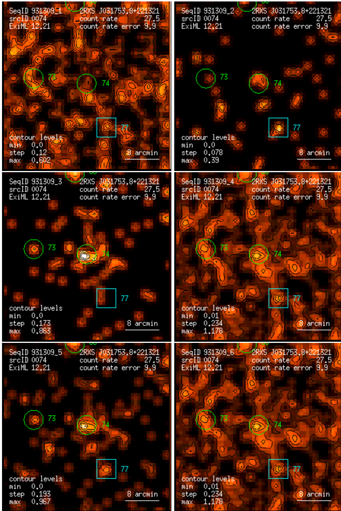
Figure 74: RASS 931309: detection 0074: band rate images, Gaussian filter: (1) PSPC channels 11 – 41, (2) 52 – 90, (3) 91 – 201, (4) 11 – 235, (5) 52 – 201, (6) 11 – 201. Broad band rates in counts/ks. Band rate contour levels in counts/ks/arcmin 2 .
