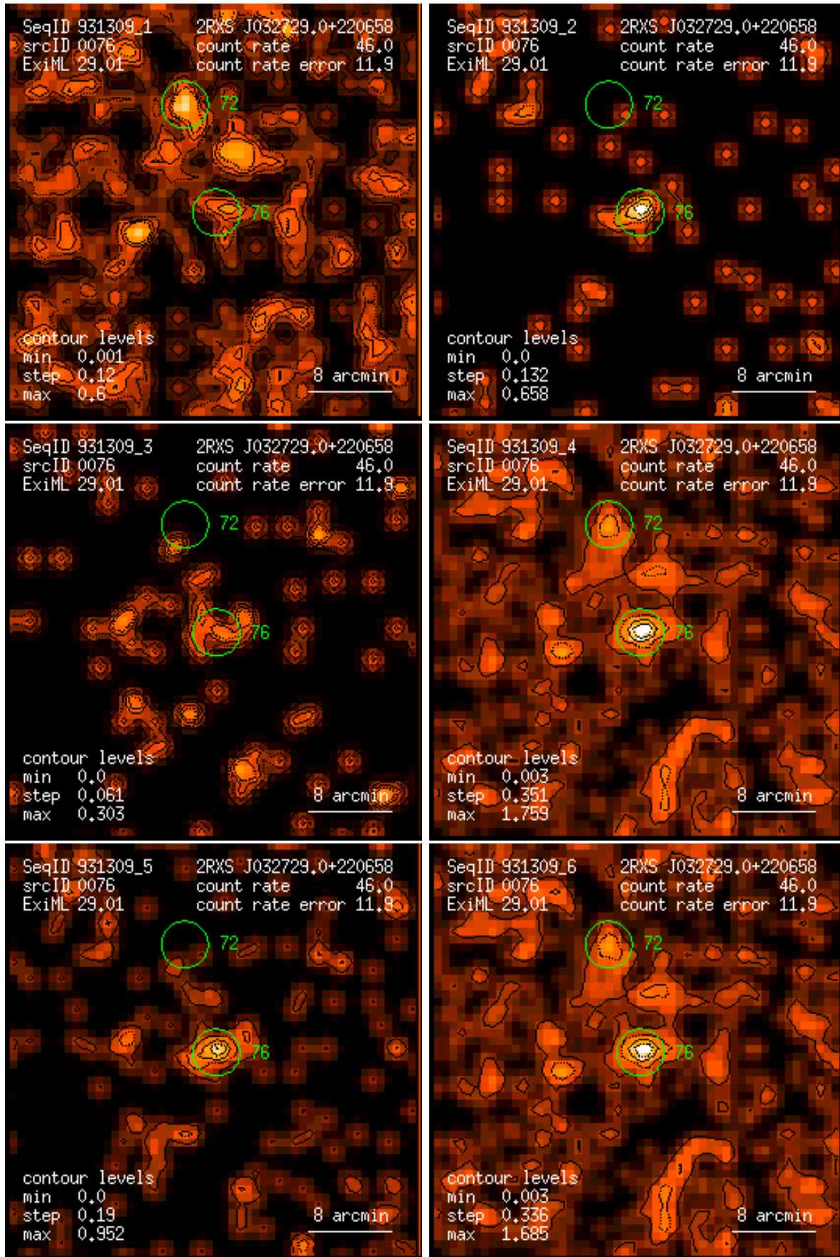
Figure 76: RASS 931309: detection 0076: band rate images, Gaussian filter: (1) PSPC channels 11 – 41, (2) 52 – 90, (3) 91 – 201, (4) 11 – 235, (5) 52 – 201, (6) 11 – 201. Broad band rates in counts/ks. Band rate contour levels in counts/ks/arcmin 2 .
