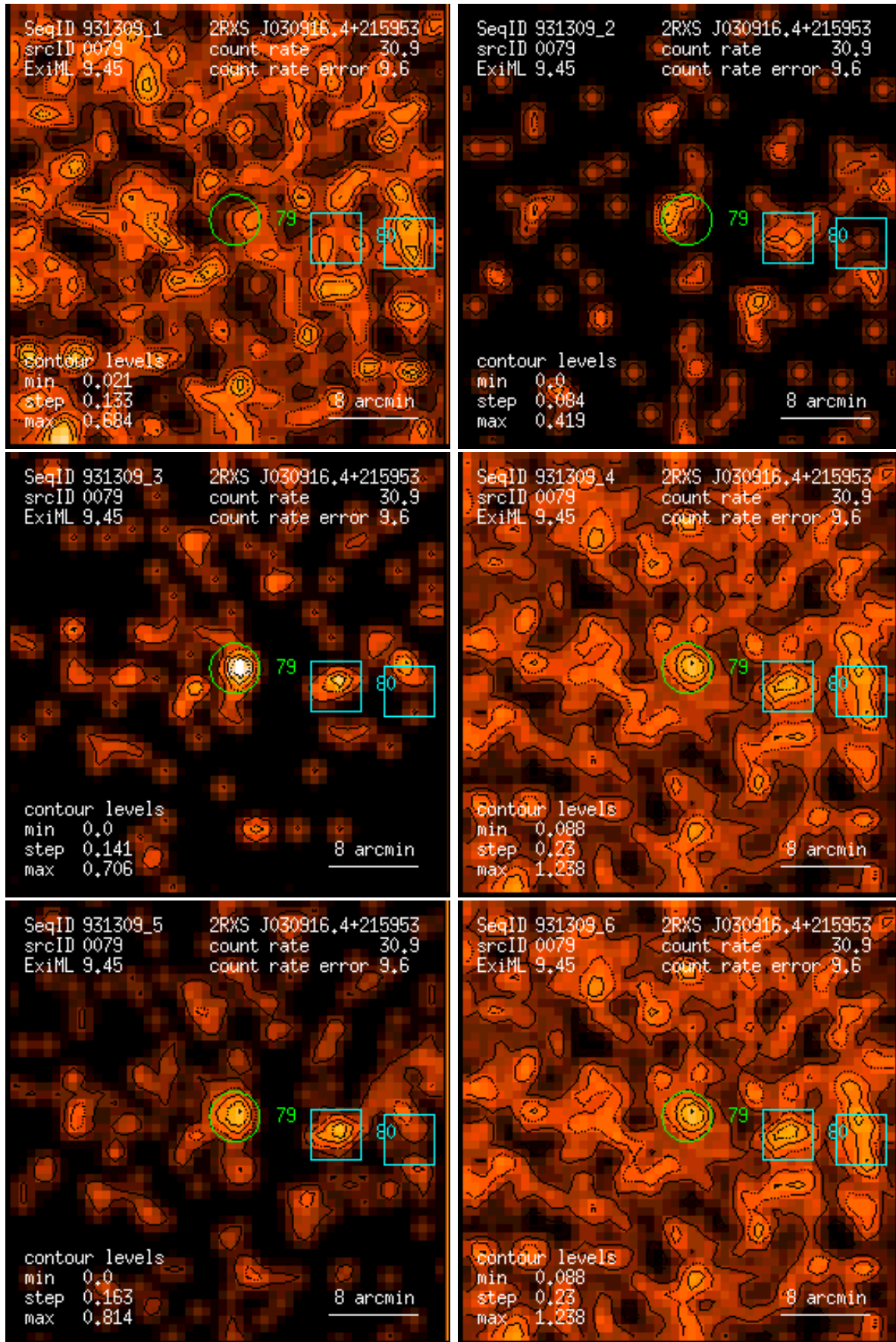
Figure 79: RASS 931309: detection 0079: band rate images, Gaussian filter: (1) PSPC channels 11 – 41, (2) 52 – 90, (3) 91 – 201, (4) 11 – 235, (5) 52 – 201, (6) 11 – 201. Broad band rates in counts/ks. Band rate contour levels in counts/ks/arcmin 2 .
