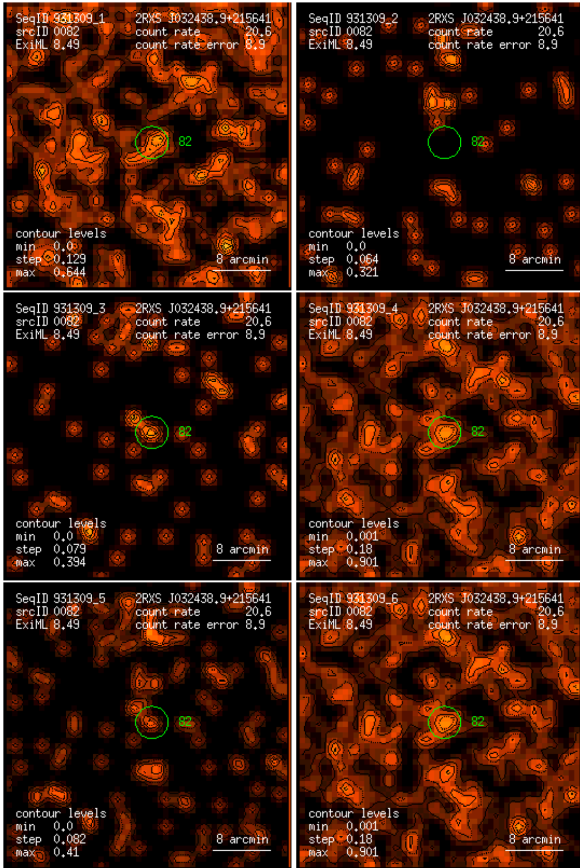
Figure 82: RASS 931309: detection 0082: band rate images, Gaussian filter: (1) PSPC channels 11 – 41, (2) 52 – 90, (3) 91 – 201, (4) 11 – 235, (5) 52 – 201, (6) 11 – 201. Broad band rates in counts/ks. Band rate contour levels in counts/ks/arcmin 2 .
