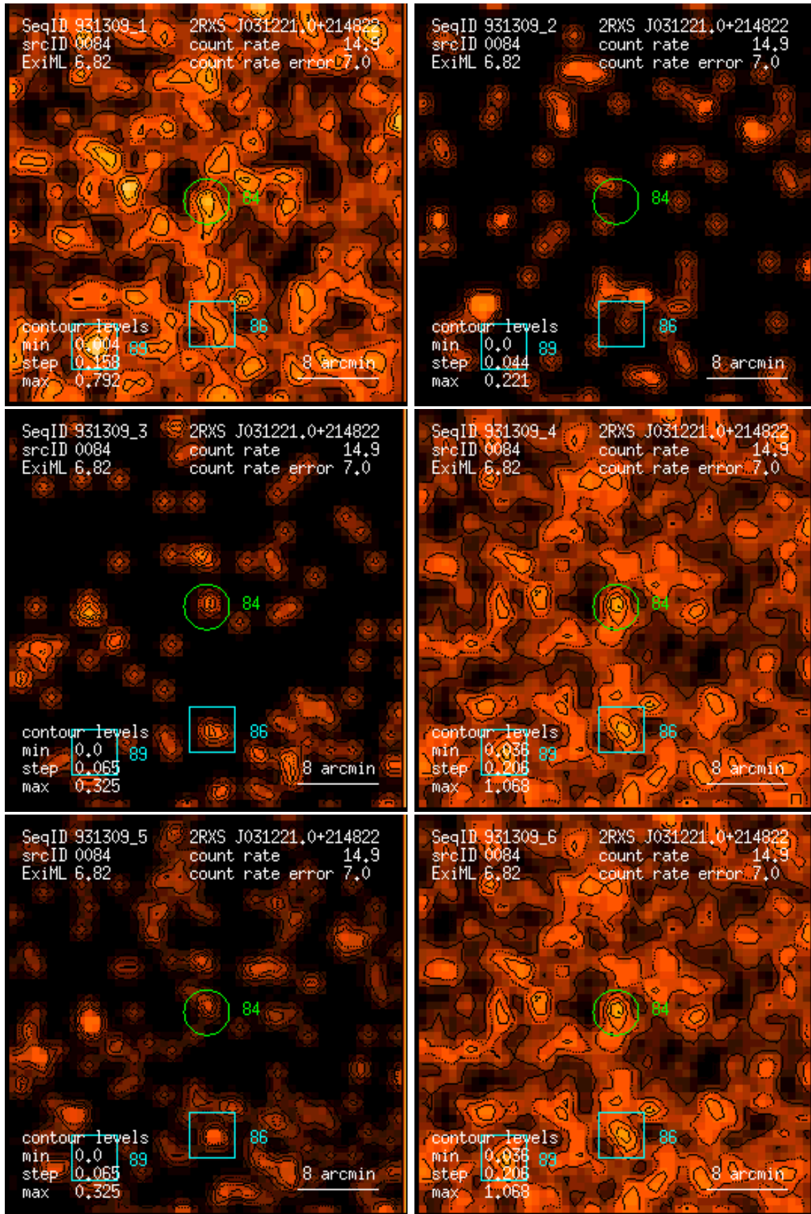
Figure 84: RASS 931309: detection 0084: band rate images, Gaussian filter: (1) PSPC channels 11 – 41, (2) 52 – 90, (3) 91 – 201, (4) 11 – 235, (5) 52 – 201, (6) 11 – 201. Broad band rates in counts/ks. Band rate contour levels in counts/ks/arcmin 2 .
