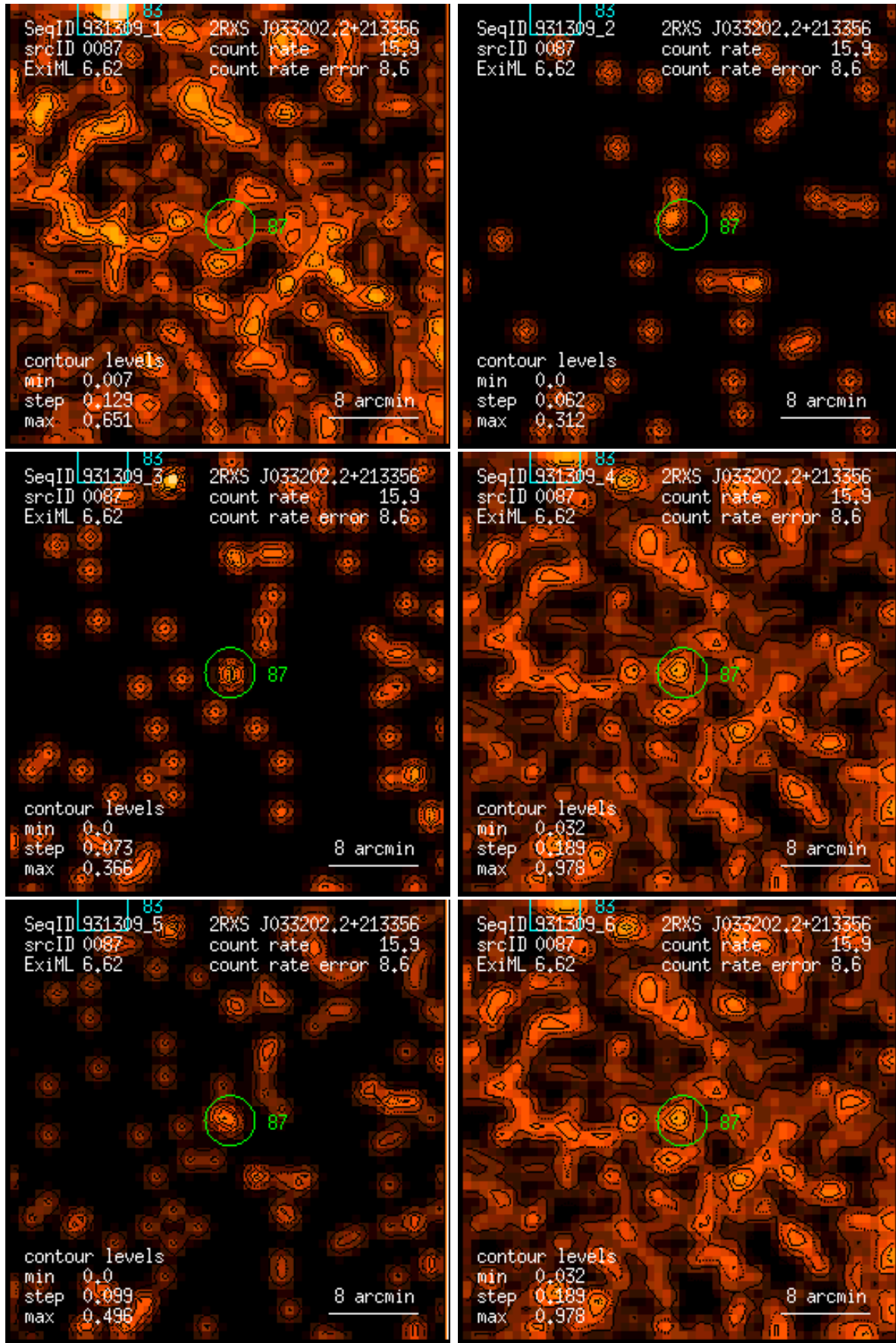
Figure 87: RASS 931309: detection 0087: band rate images, Gaussian filter: (1) PSPC channels 11 – 41, (2) 52 – 90, (3) 91 – 201, (4) 11 – 235, (5) 52 – 201, (6) 11 – 201. Broad band rates in counts/ks. Band rate contour levels in counts/ks/arcmin 2 .
