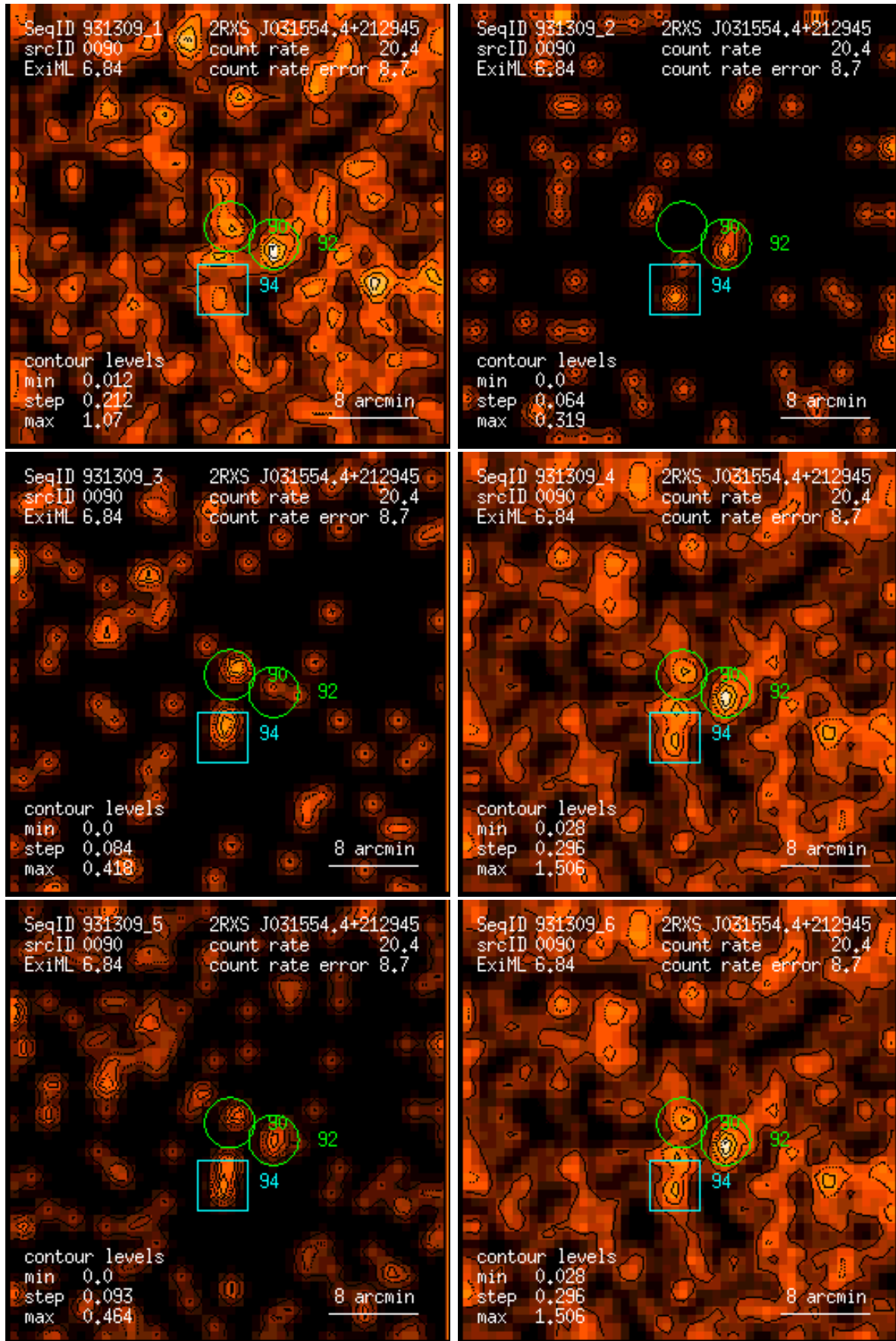
Figure 90: RASS 931309: detection 0090: band rate images, Gaussian filter: (1) PSPC channels 11 – 41, (2) 52 – 90, (3) 91 – 201, (4) 11 – 235, (5) 52 – 201, (6) 11 – 201. Broad band rates in counts/ks. Band rate contour levels in counts/ks/arcmin 2 .
