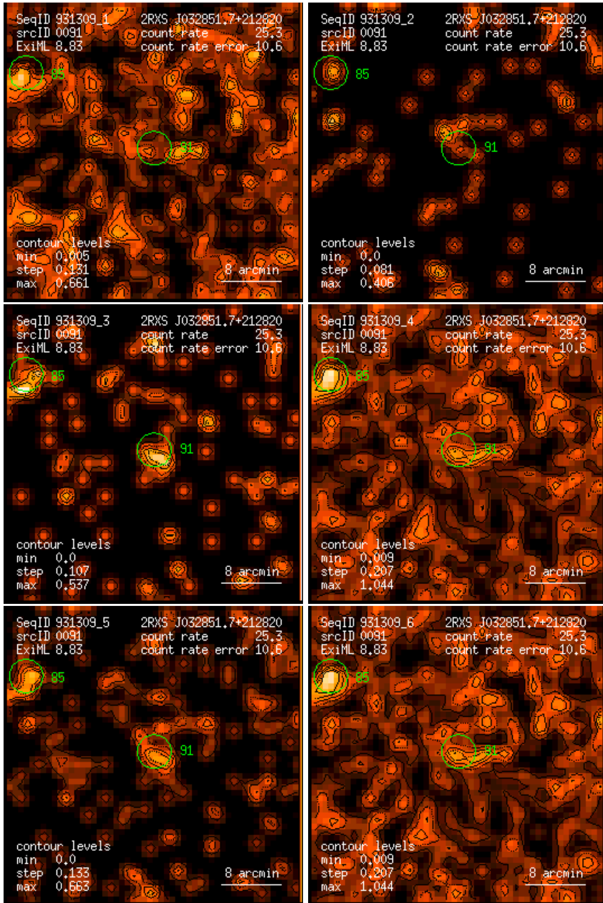
Figure 91: RASS 931309: detection 0091: band rate images, Gaussian filter: (1) PSPC channels 11 – 41, (2) 52 – 90, (3) 91 – 201, (4) 11 – 235, (5) 52 – 201, (6) 11 – 201. Broad band rates in counts/ks. Band rate contour levels in counts/ks/arcmin 2 .
