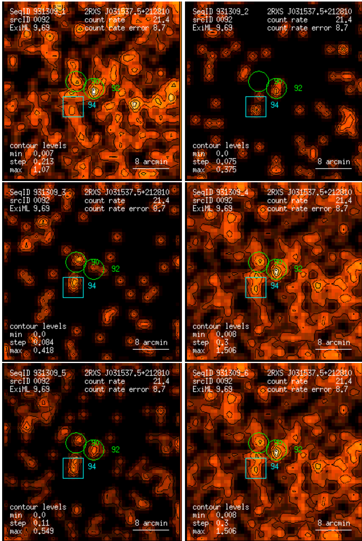
Figure 92: RASS 931309: detection 0092: band rate images, Gaussian filter: (1) PSPC channels 11 – 41, (2) 52 – 90, (3) 91 – 201, (4) 11 – 235, (5) 52 – 201, (6) 11 – 201. Broad band rates in counts/ks. Band rate contour levels in counts/ks/arcmin 2 .
