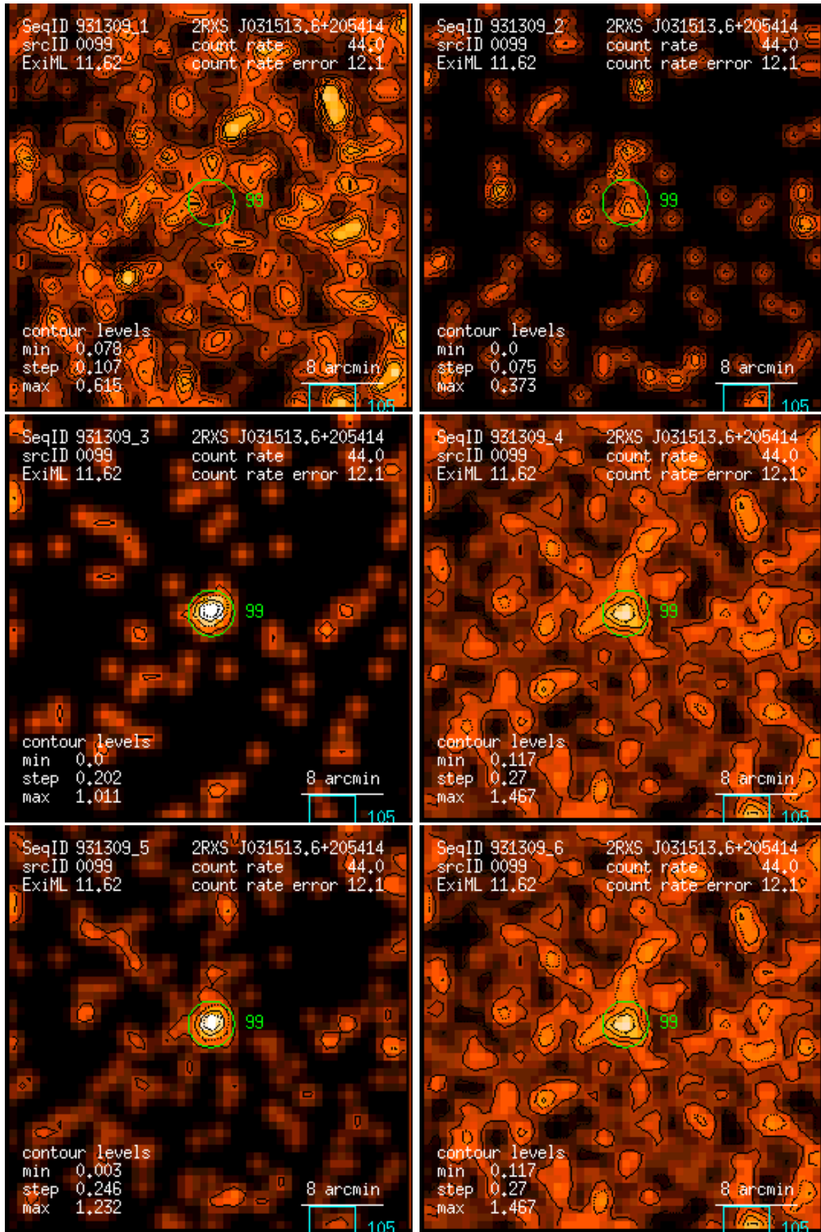
Figure 99: RASS 931309: detection 0099: band rate images, Gaussian filter: (1) PSPC channels 11 – 41, (2) 52 – 90, (3) 91 – 201, (4) 11 – 235, (5) 52 – 201, (6) 11 – 201. Broad band rates in counts/ks. Band rate contour levels in counts/ks/arcmin 2 .
