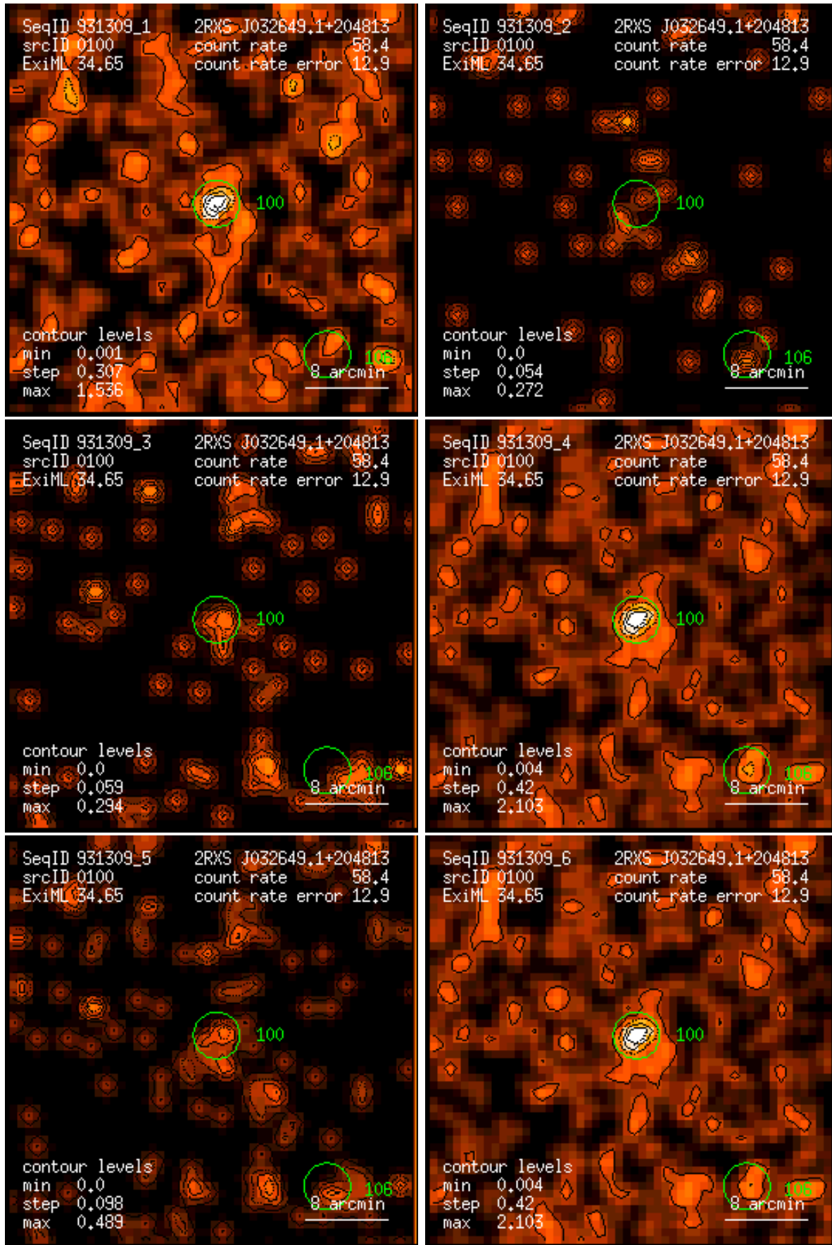
Figure 100: RASS 931309: detection 0100: band rate images, Gaussian filter: (1) PSPC channels 11 – 41, (2) 52 – 90, (3) 91 – 201, (4) 11 – 235, (5) 52 – 201, (6) 11 – 201. Broad band rates in counts/ks. Band rate contour levels in counts/ks/arcmin 2 .
