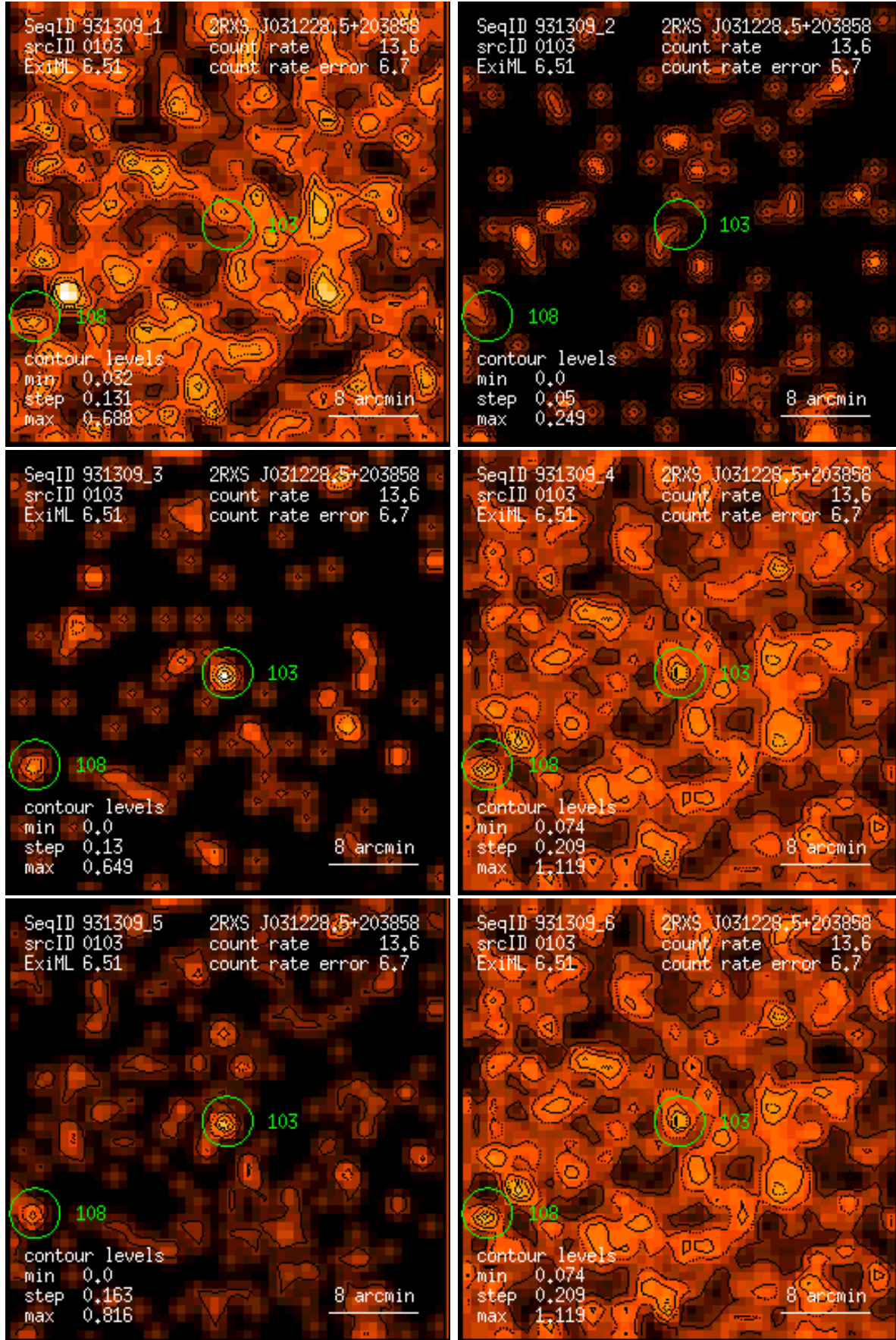
Figure 103: RASS 931309: detection 0103: band rate images, Gaussian filter: (1) PSPC channels 11 – 41, (2) 52 – 90, (3) 91 – 201, (4) 11 – 235, (5) 52 – 201, (6) 11 – 201. Broad band rates in counts/ks. Band rate contour levels in counts/ks/arcmin 2 .
