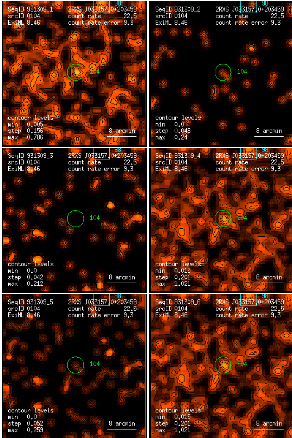
Figure 104: RASS 931309: detection 0104: band rate images, Gaussian filter: (1) PSPC channels 11 – 41, (2) 52 – 90, (3) 91 – 201, (4) 11 – 235, (5) 52 – 201, (6) 11 – 201. Broad band rates in counts/ks. Band rate contour levels in counts/ks/arcmin 2 .
