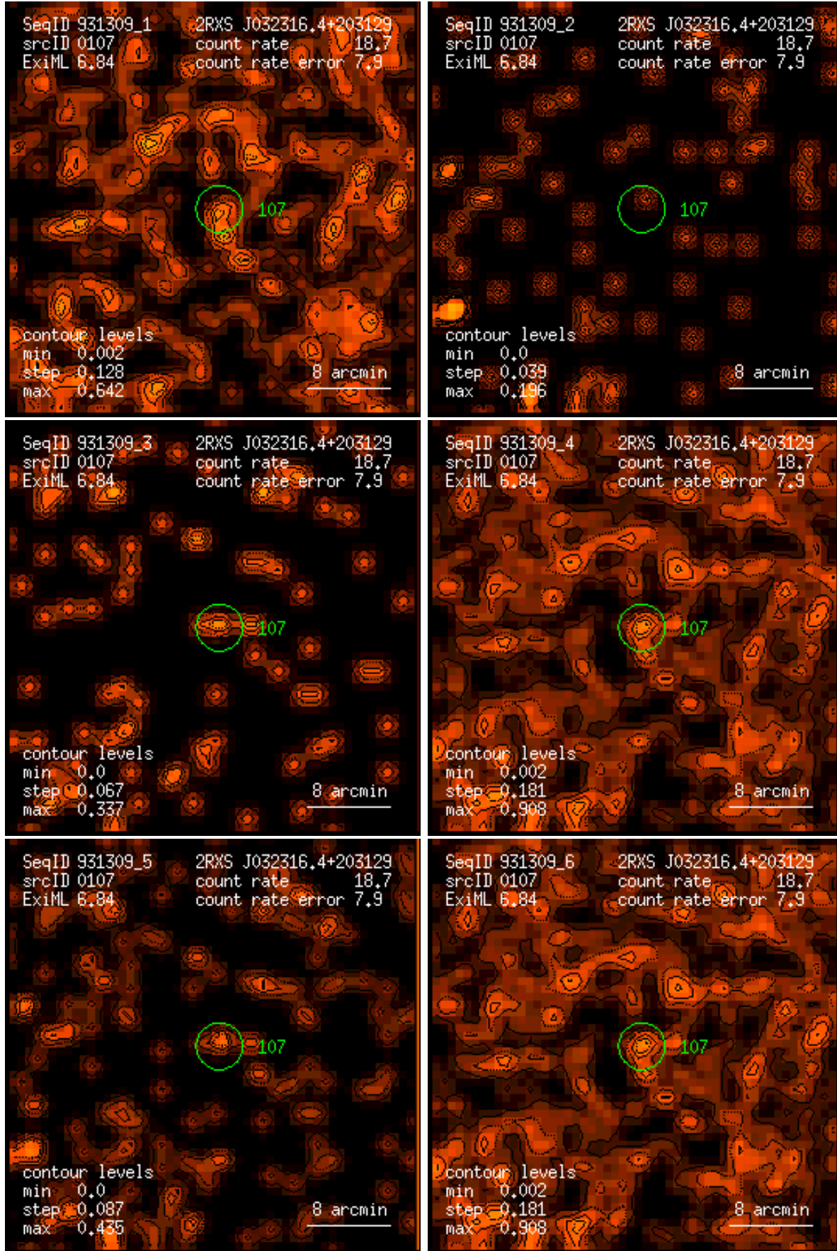
Figure 107: RASS 931309: detection 0107: band rate images, Gaussian filter: (1) PSPC channels 11 – 41, (2) 52 – 90, (3) 91 – 201, (4) 11 – 235, (5) 52 – 201, (6) 11 – 201. Broad band rates in counts/ks. Band rate contour levels in counts/ks/arcmin 2 .
