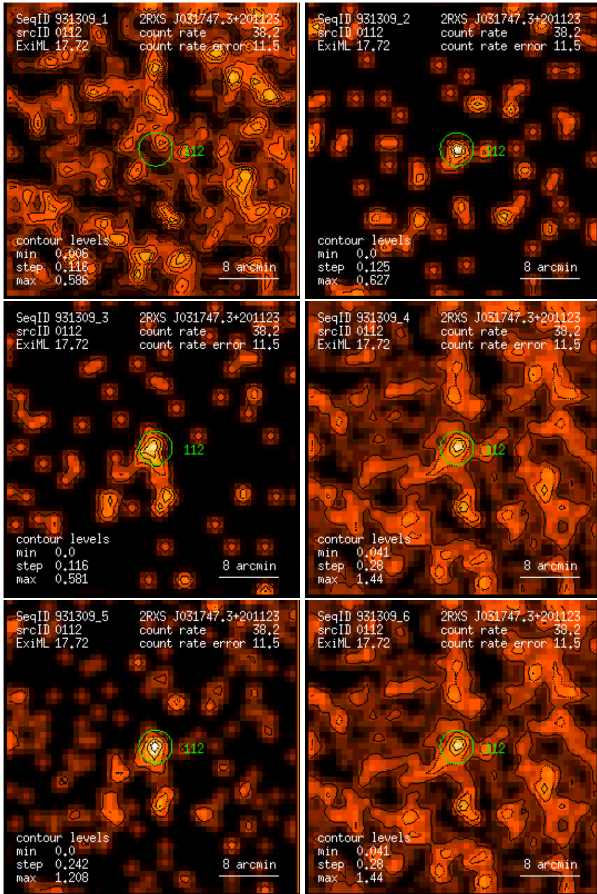
Figure 112: RASS 931309: detection 0112: band rate images, Gaussian filter: (1) PSPC channels 11 – 41, (2) 52 – 90, (3) 91 – 201, (4) 11 – 235, (5) 52 – 201, (6) 11 – 201. Broad band rates in counts/ks. Band rate contour levels in counts/ks/arcmin 2 .
