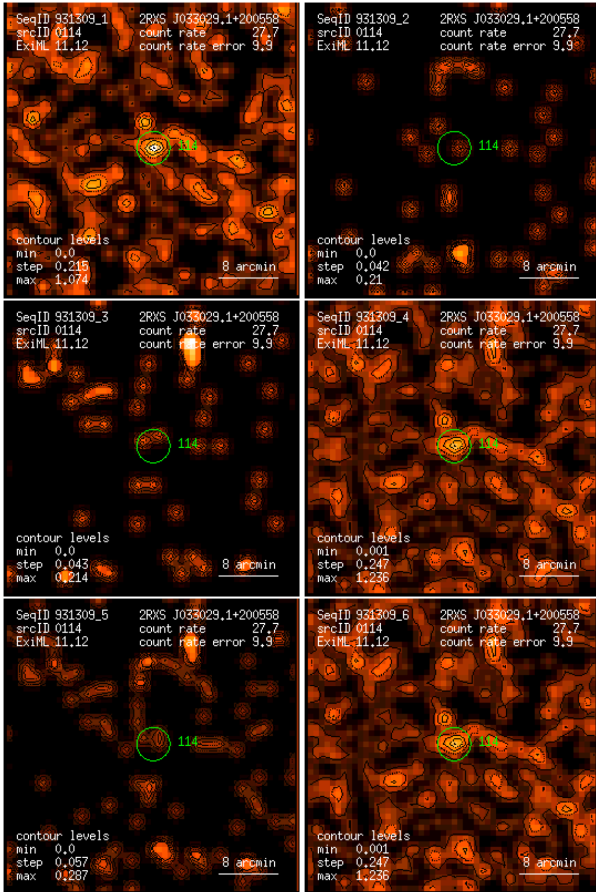
Figure 114: RASS 931309: detection 0114: band rate images, Gaussian filter: (1) PSPC channels 11 – 41, (2) 52 – 90, (3) 91 – 201, (4) 11 – 235, (5) 52 – 201, (6) 11 – 201. Broad band rates in counts/ks. Band rate contour levels in counts/ks/arcmin 2 .
