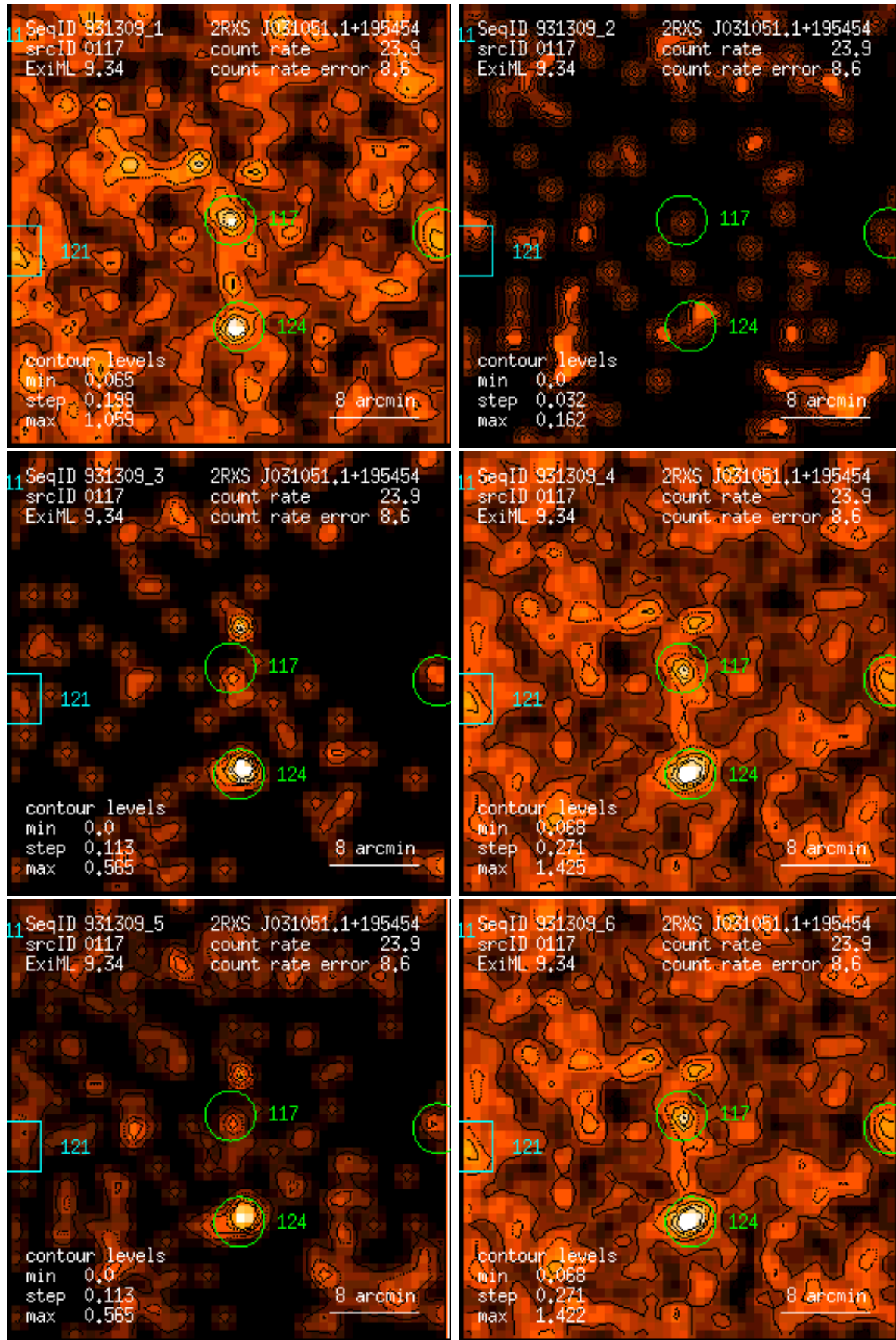
Figure 117: RASS 931309: detection 0117: band rate images, Gaussian filter: (1) PSPC channels 11 – 41, (2) 52 – 90, (3) 91 – 201, (4) 11 – 235, (5) 52 – 201, (6) 11 – 201. Broad band rates in counts/ks. Band rate contour levels in counts/ks/arcmin 2 .
