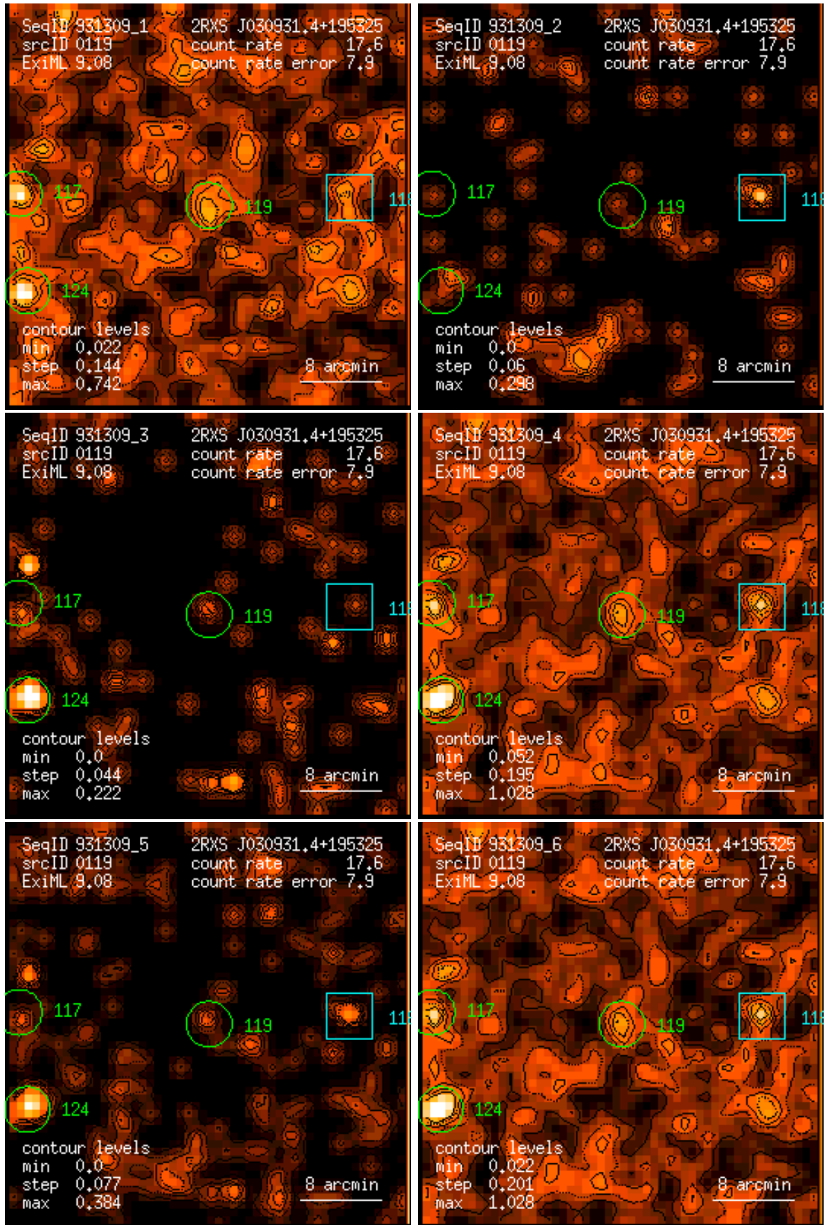
Figure 119: RASS 931309: detection 0119: band rate images, Gaussian filter: (1) PSPC channels 11 – 41, (2) 52 – 90, (3) 91 – 201, (4) 11 – 235, (5) 52 – 201, (6) 11 – 201. Broad band rates in counts/ks. Band rate contour levels in counts/ks/arcmin 2 .
