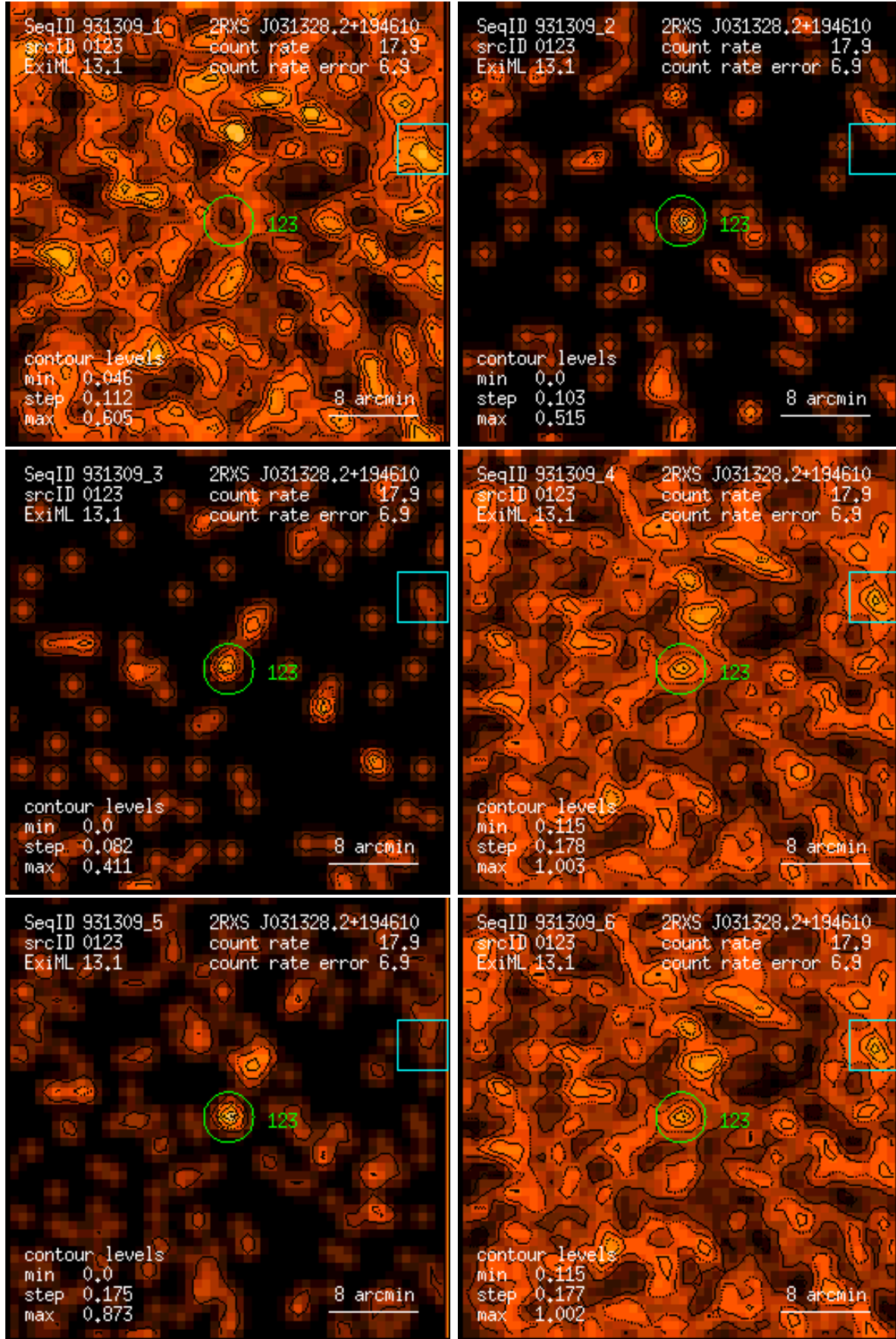
Figure 123: RASS 931309: detection 0123: band rate images, Gaussian filter: (1) PSPC channels 11 – 41, (2) 52 – 90, (3) 91 – 201, (4) 11 – 235, (5) 52 – 201, (6) 11 – 201. Broad band rates in counts/ks. Band rate contour levels in counts/ks/arcmin 2 .
