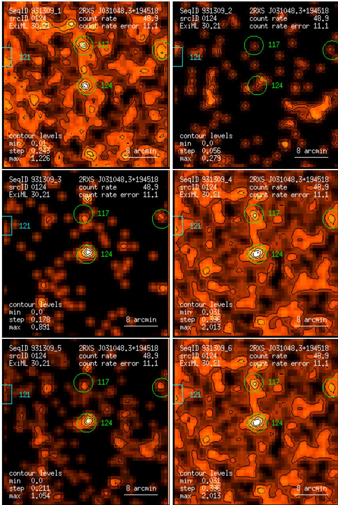
Figure 124: RASS 931309: detection 0124: band rate images, Gaussian filter: (1) PSPC channels 11 – 41, (2) 52 – 90, (3) 91 – 201, (4) 11 – 235, (5) 52 – 201, (6) 11 – 201. Broad band rates in counts/ks. Band rate contour levels in counts/ks/arcmin 2 .
