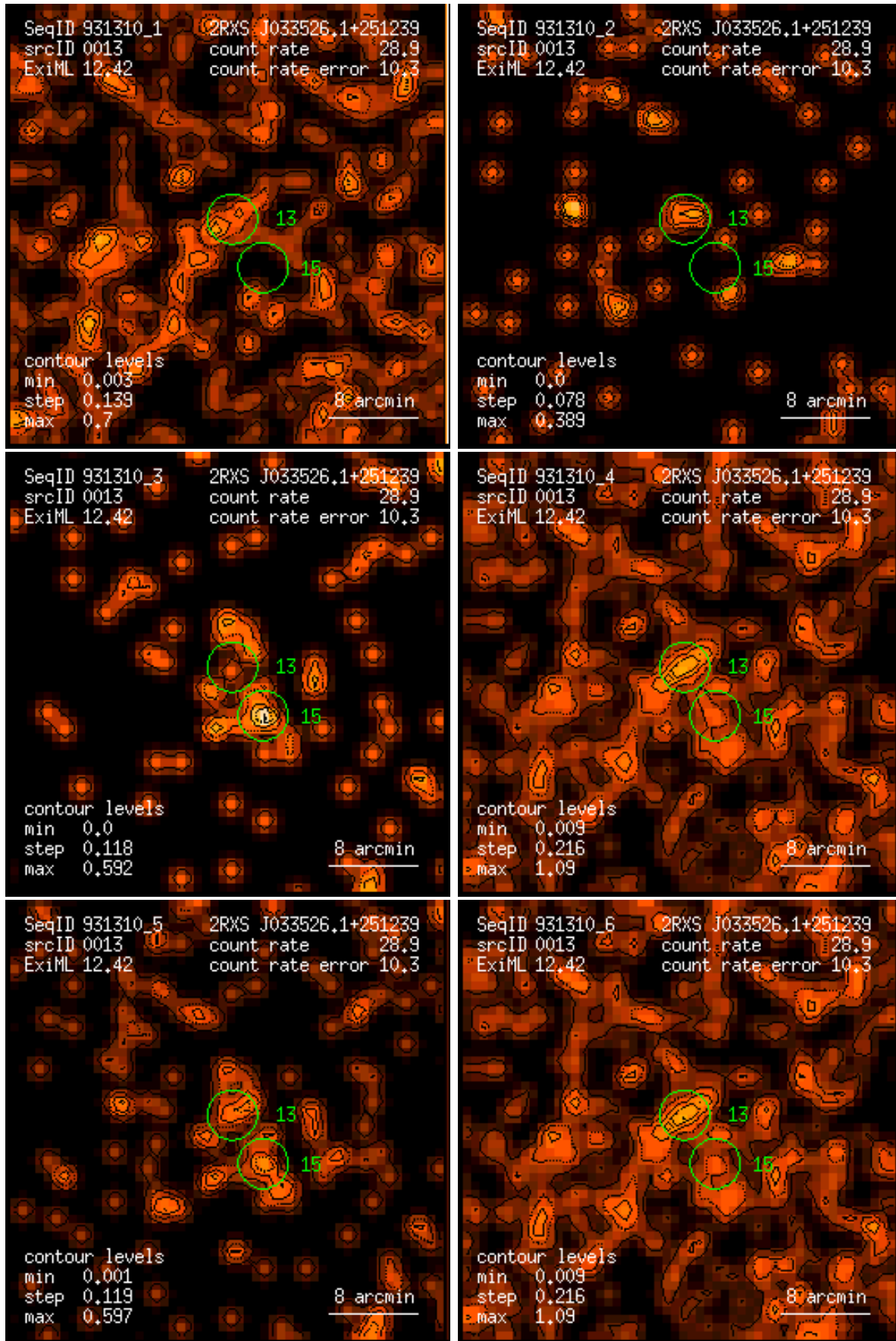
Figure 13: RASS 931310: detection 0013: band rate images, Gaussian filter: (1) PSPC channels 11 – 41, (2) 52 – 90, (3) 91 – 201, (4) 11 – 235, (5) 52 – 201, (6) 11 – 201. Broad band rates in counts/ks. Band rate contour levels in counts/ks/arcmin 2 .
