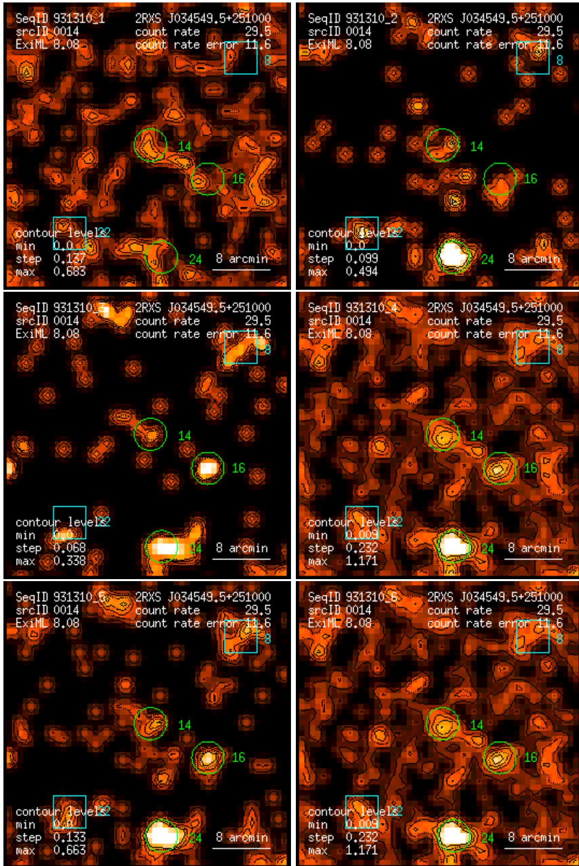
Figure 14: RASS 931310: detection 0014: band rate images, Gaussian filter: (1) PSPC channels 11 – 41, (2) 52 – 90, (3) 91 – 201, (4) 11 – 235, (5) 52 – 201, (6) 11 – 201. Broad band rates in counts/ks. Band rate contour levels in counts/ks/arcmin 2 .
