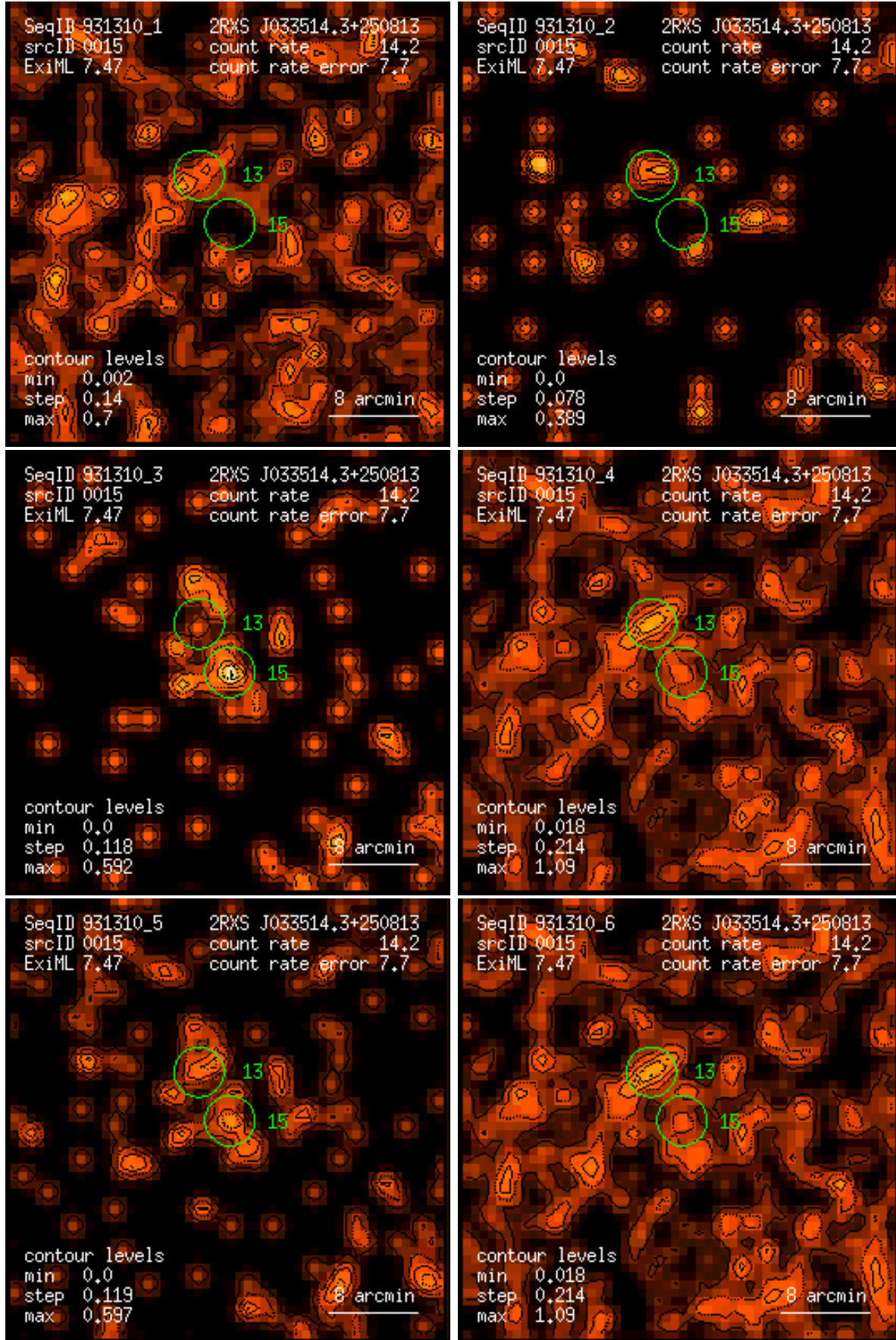
Figure 15: RASS 931310: detection 0015: band rate images, Gaussian filter: (1) PSPC channels 11 – 41, (2) 52 – 90, (3) 91 – 201, (4) 11 – 235, (5) 52 – 201, (6) 11 – 201. Broad band rates in counts/ks. Band rate contour levels in counts/ks/arcmin 2 .
