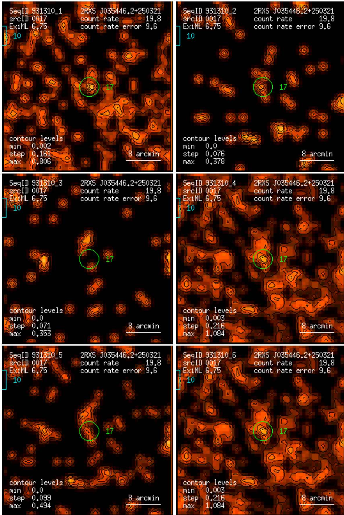
Figure 17: RASS 931310: detection 0017: band rate images, Gaussian filter: (1) PSPC channels 11 – 41, (2) 52 – 90, (3) 91 – 201, (4) 11 – 235, (5) 52 – 201, (6) 11 – 201. Broad band rates in counts/ks. Band rate contour levels in counts/ks/arcmin 2 .
