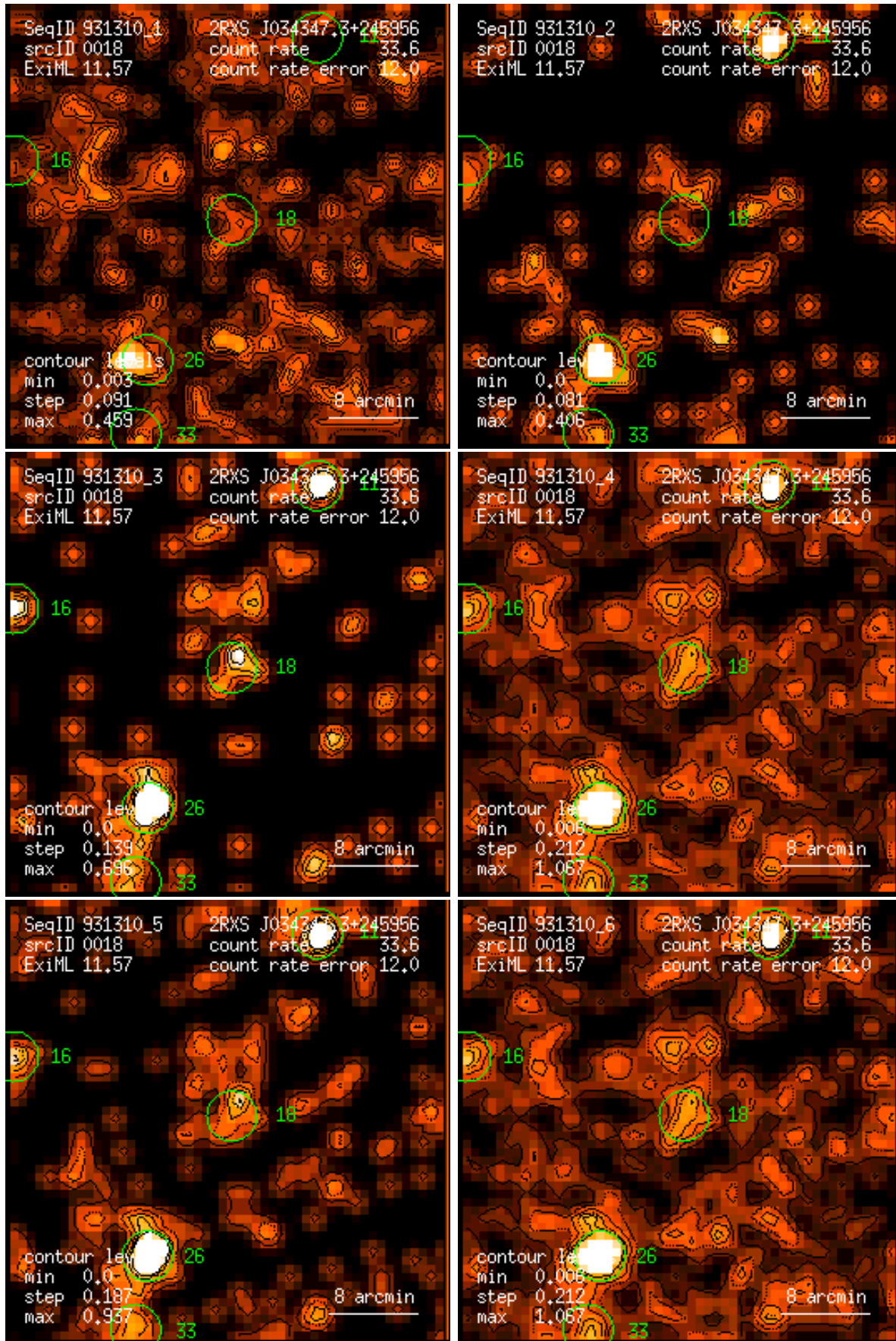
Figure 18: RASS 931310: detection 0018: band rate images, Gaussian filter: (1) PSPC channels 11 – 41, (2) 52 – 90, (3) 91 – 201, (4) 11 – 235, (5) 52 – 201, (6) 11 – 201. Broad band rates in counts/ks. Band rate contour levels in counts/ks/arcmin 2 .
