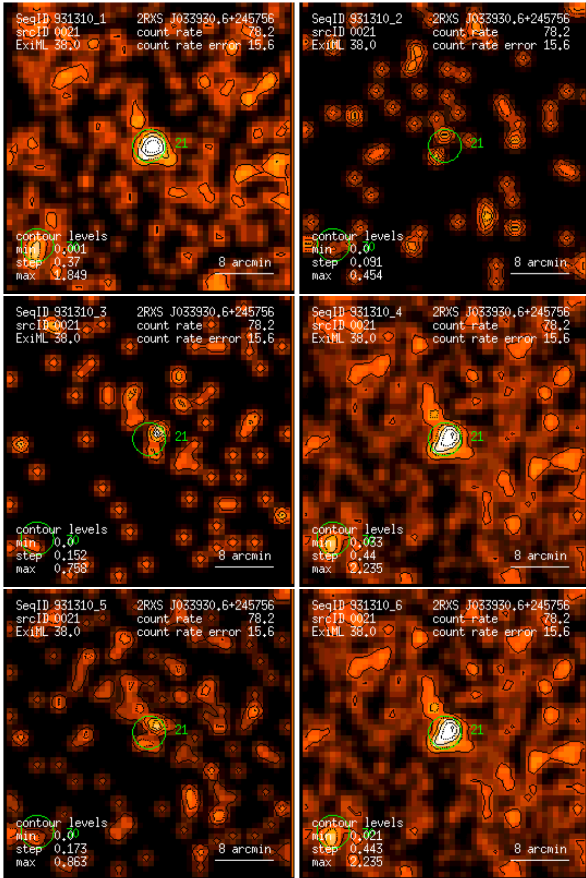
Figure 21: RASS 931310: detection 0021: band rate images, Gaussian filter: (1) PSPC channels 11 – 41, (2) 52 – 90, (3) 91 – 201, (4) 11 – 235, (5) 52 – 201, (6) 11 – 201. Broad band rates in counts/ks. Band rate contour levels in counts/ks/arcmin 2 .
