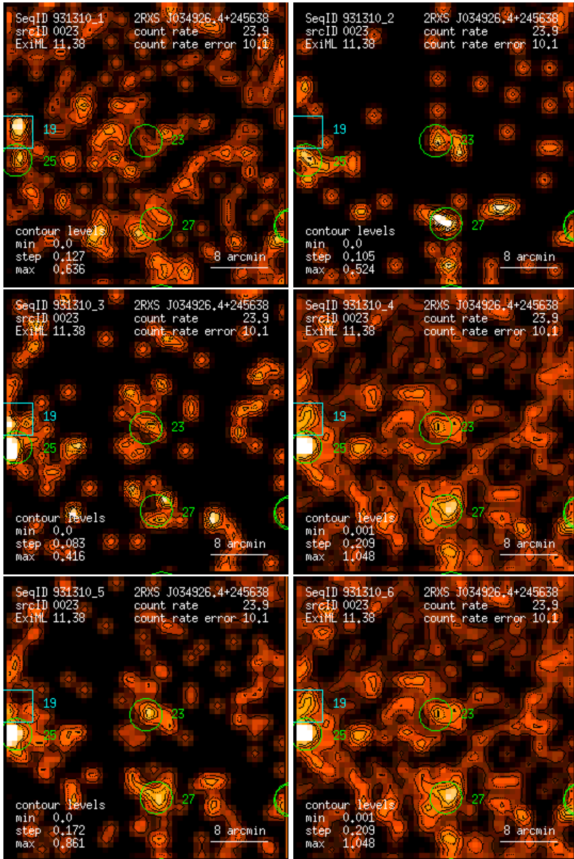
Figure 23: RASS 931310: detection 0023: band rate images, Gaussian filter: (1) PSPC channels 11 – 41, (2) 52 – 90, (3) 91 – 201, (4) 11 – 235, (5) 52 – 201, (6) 11 – 201. Broad band rates in counts/ks. Band rate contour levels in counts/ks/arcmin 2 .
