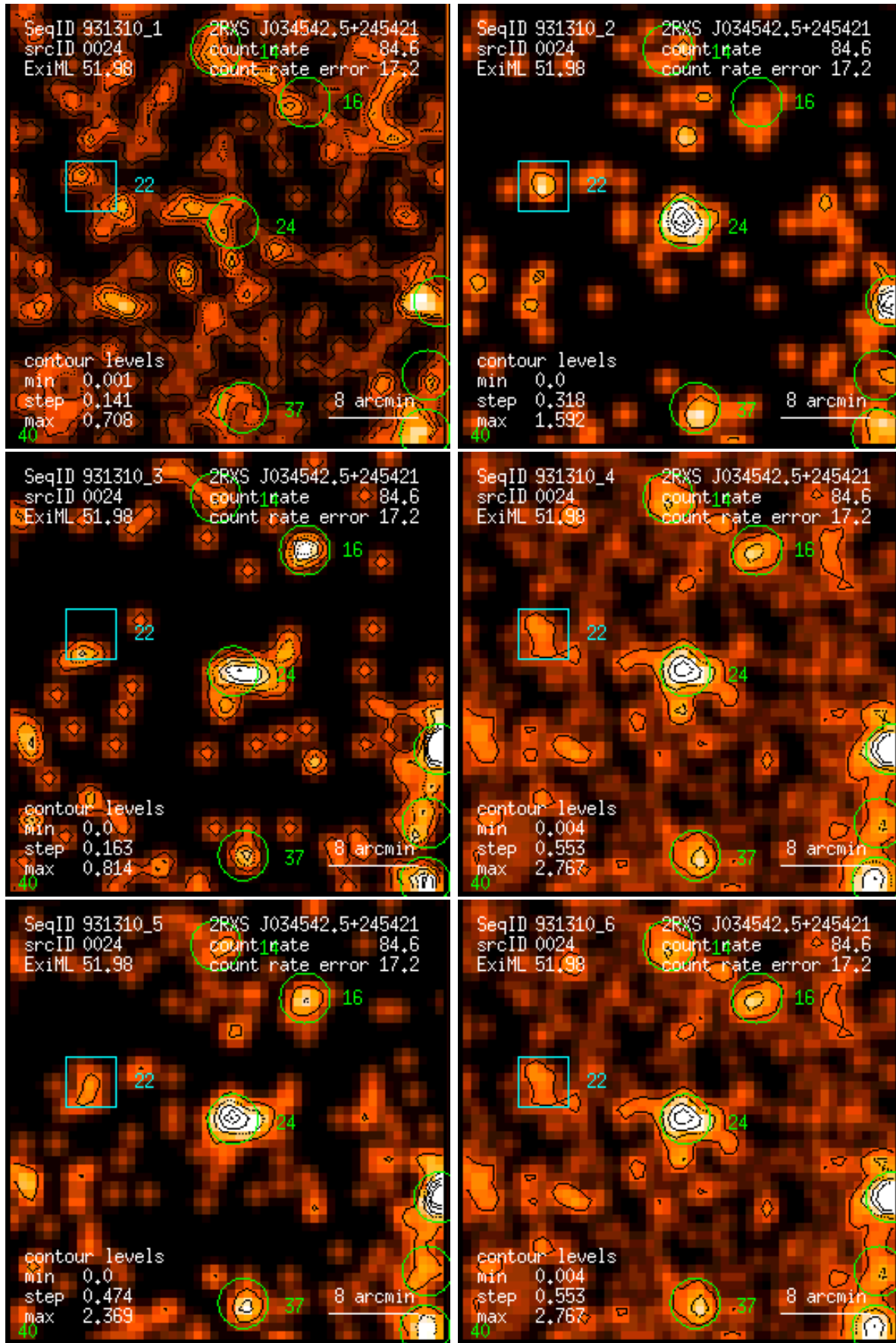
Figure 24: RASS 931310: detection 0024: band rate images, Gaussian filter: (1) PSPC channels 11 – 41, (2) 52 – 90, (3) 91 – 201, (4) 11 – 235, (5) 52 – 201, (6) 11 – 201. Broad band rates in counts/ks. Band rate contour levels in counts/ks/arcmin 2 .
