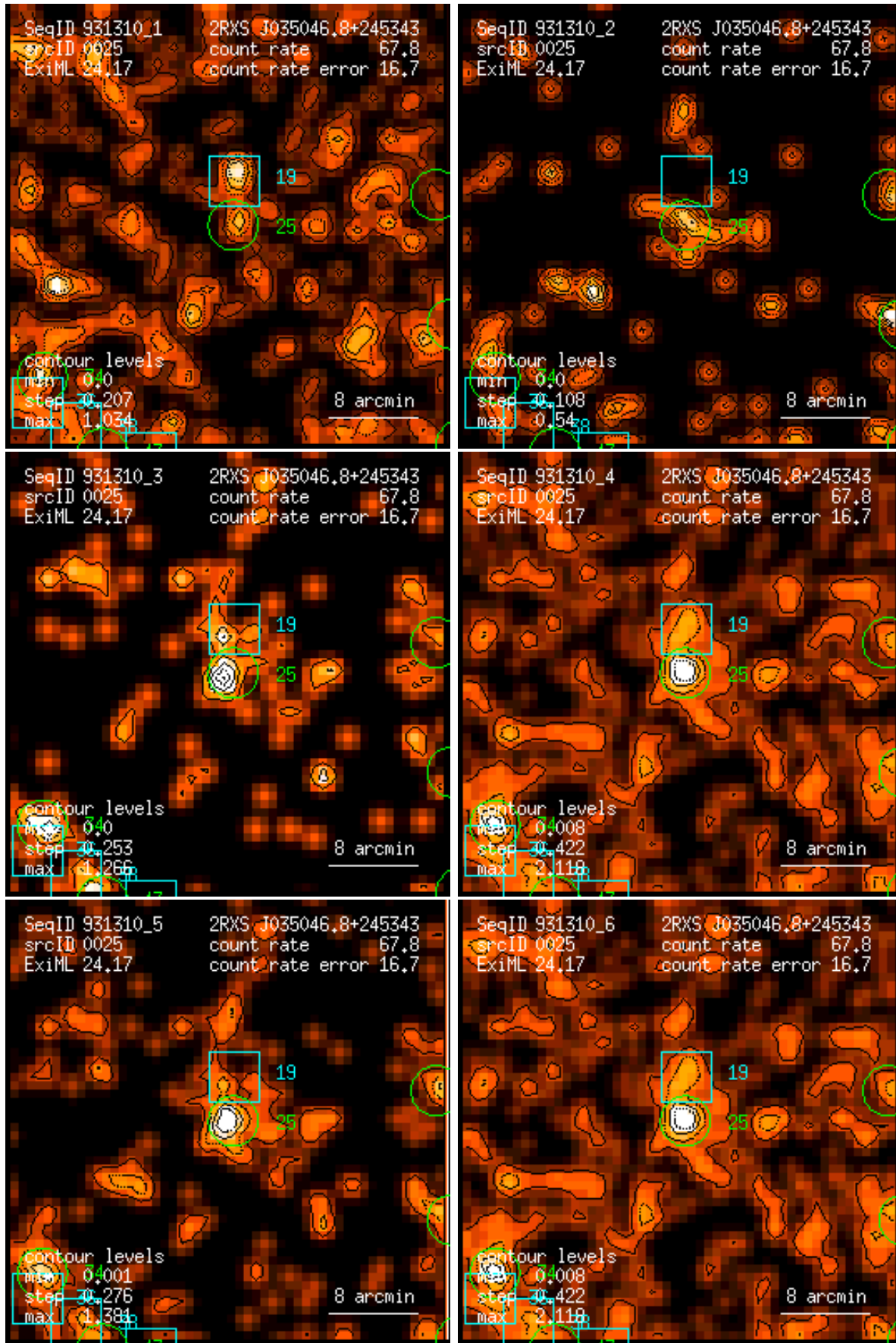
Figure 25: RASS 931310: detection 0025: band rate images, Gaussian filter: (1) PSPC channels 11 – 41, (2) 52 – 90, (3) 91 – 201, (4) 11 – 235, (5) 52 – 201, (6) 11 – 201. Broad band rates in counts/ks. Band rate contour levels in counts/ks/arcmin 2 .
