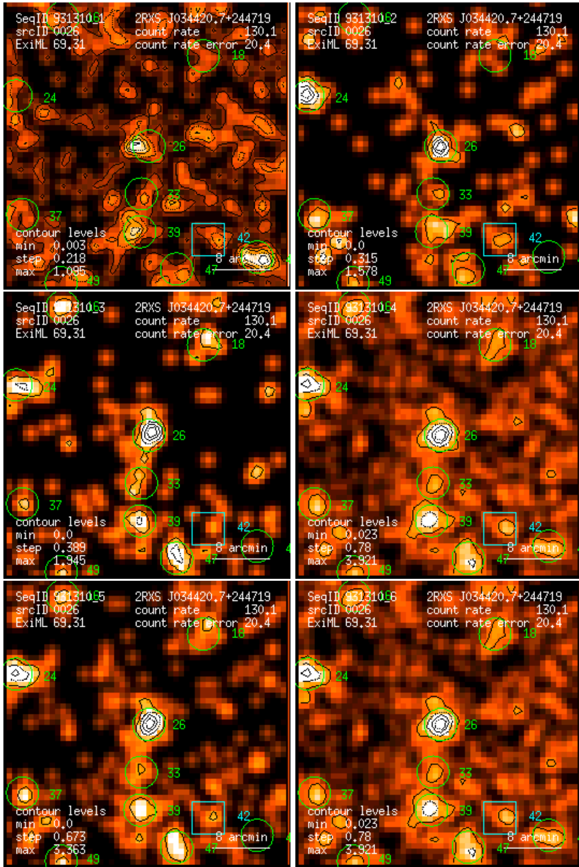
Figure 26: RASS 931310: detection 0026: band rate images, Gaussian filter: (1) PSPC channels 11 – 41, (2) 52 – 90, (3) 91 – 201, (4) 11 – 235, (5) 52 – 201, (6) 11 – 201. Broad band rates in counts/ks. Band rate contour levels in counts/ks/arcmin 2 .
