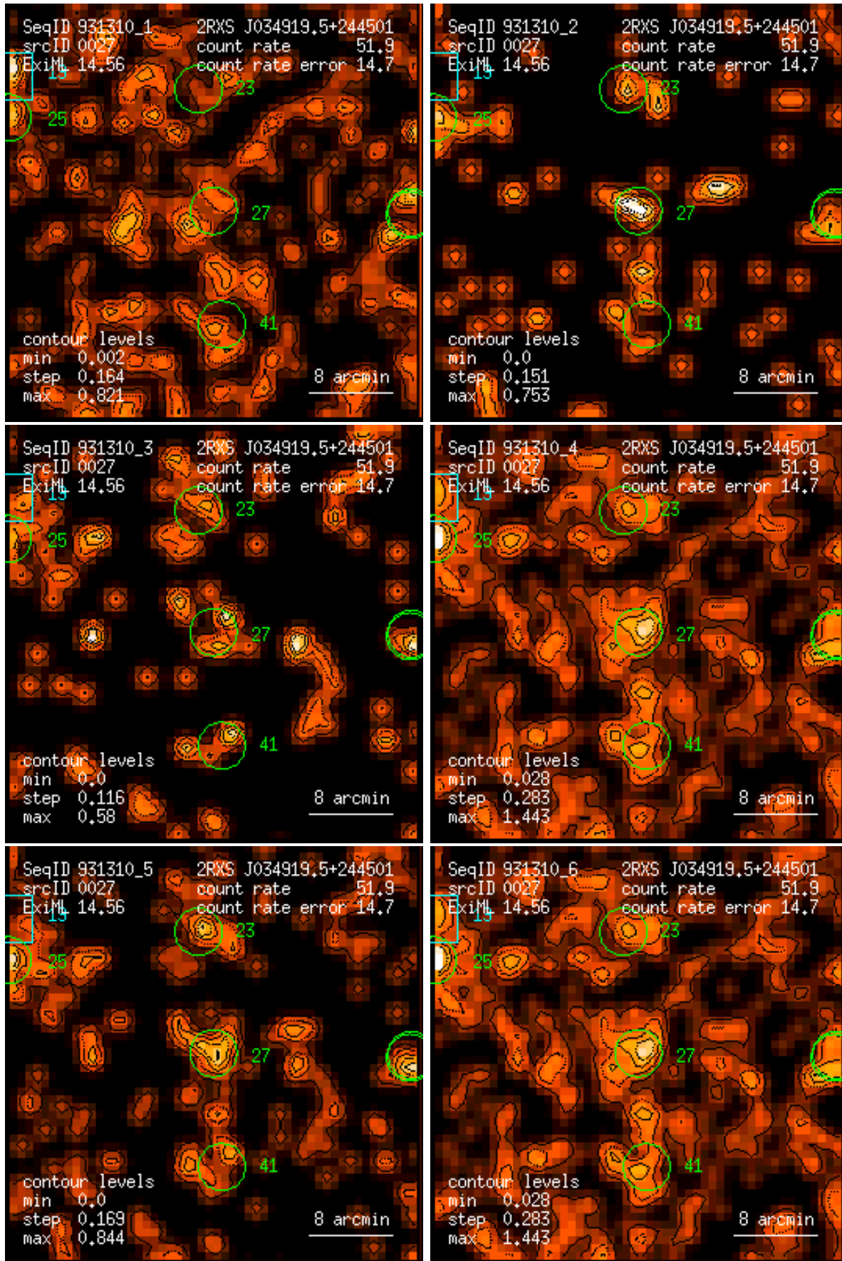
Figure 27: RASS 931310: detection 0027: band rate images, Gaussian filter: (1) PSPC channels 11 – 41, (2) 52 – 90, (3) 91 – 201, (4) 11 – 235, (5) 52 – 201, (6) 11 – 201. Broad band rates in counts/ks. Band rate contour levels in counts/ks/arcmin 2 .
