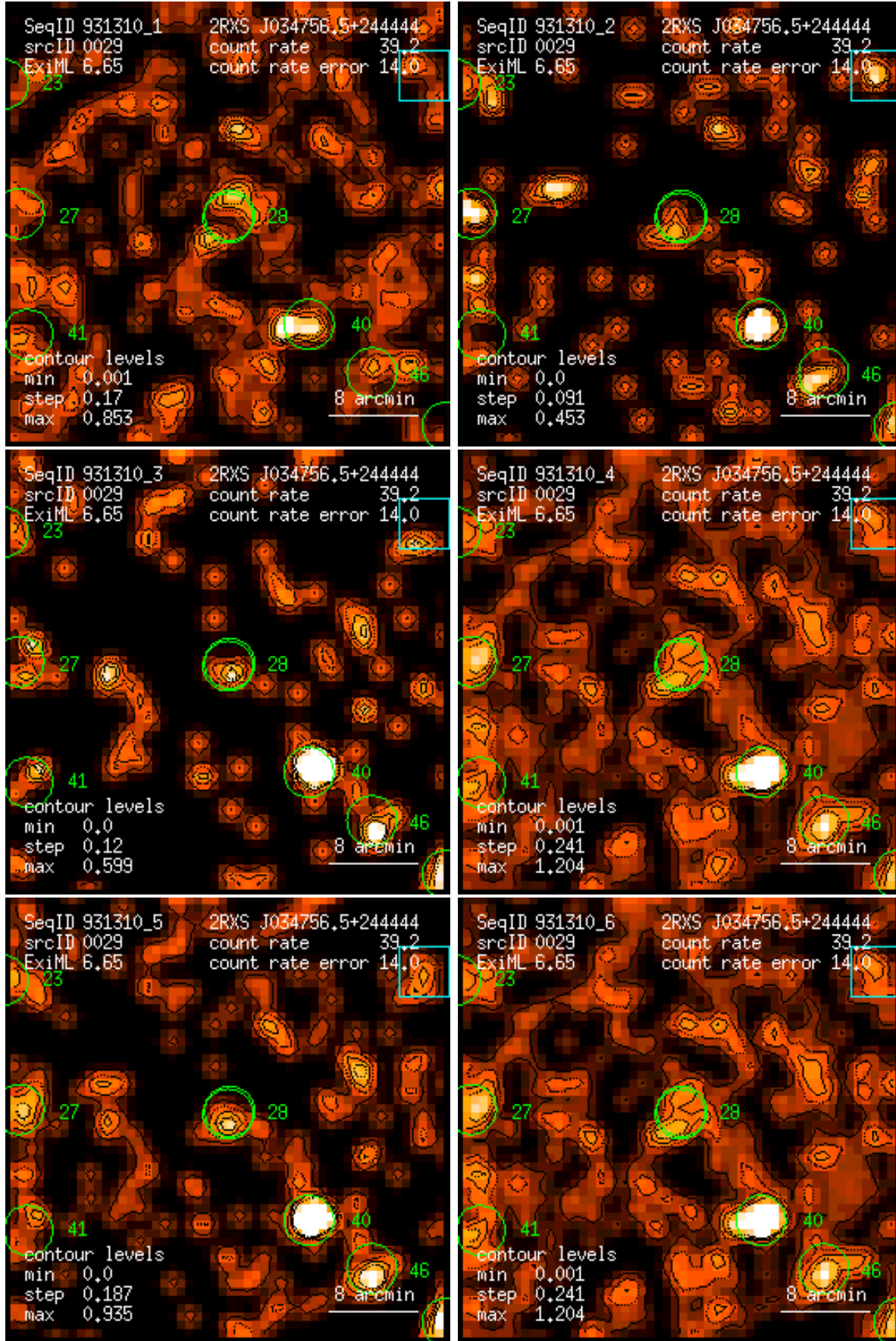
Figure 29: RASS 931310: detection 0029: band rate images, Gaussian filter: (1) PSPC channels 11 – 41, (2) 52 – 90, (3) 91 – 201, (4) 11 – 235, (5) 52 – 201, (6) 11 – 201. Broad band rates in counts/ks. Band rate contour levels in counts/ks/arcmin 2 .
