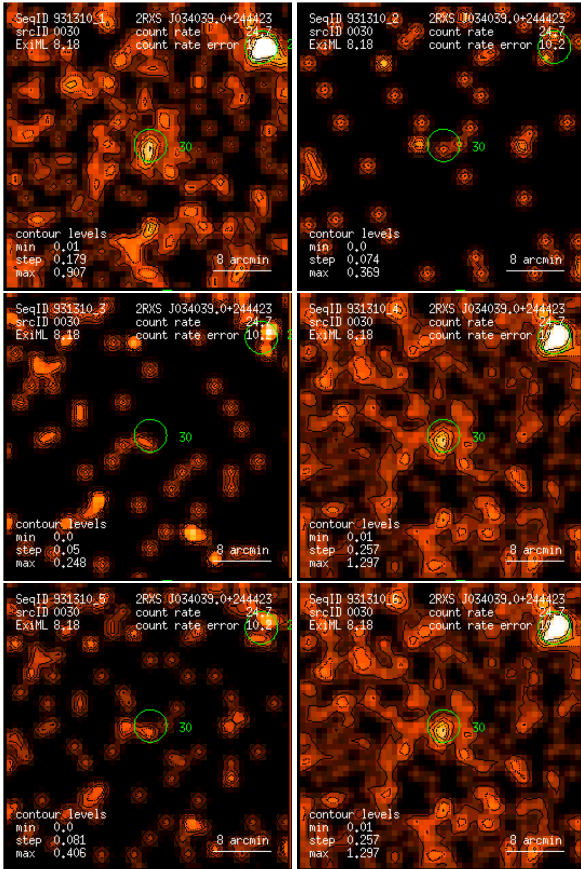
Figure 30: RASS 931310: detection 0030: band rate images, Gaussian filter: (1) PSPC channels 11 – 41, (2) 52 – 90, (3) 91 – 201, (4) 11 – 235, (5) 52 – 201, (6) 11 – 201. Broad band rates in counts/ks. Band rate contour levels in counts/ks/arcmin 2 .
